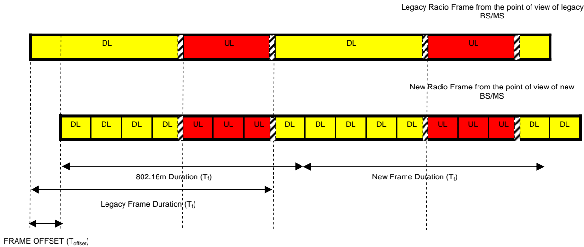
3 4 Figure 12 Relative position of the new and legacy radio frames (example TDD duplex scheme) → proposal-1 5 6
