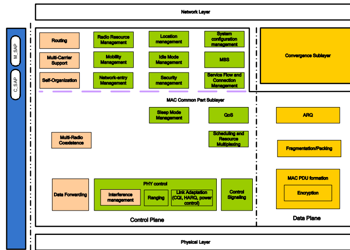
Figure 4 The IEEE 802.16m Protocol Structure
