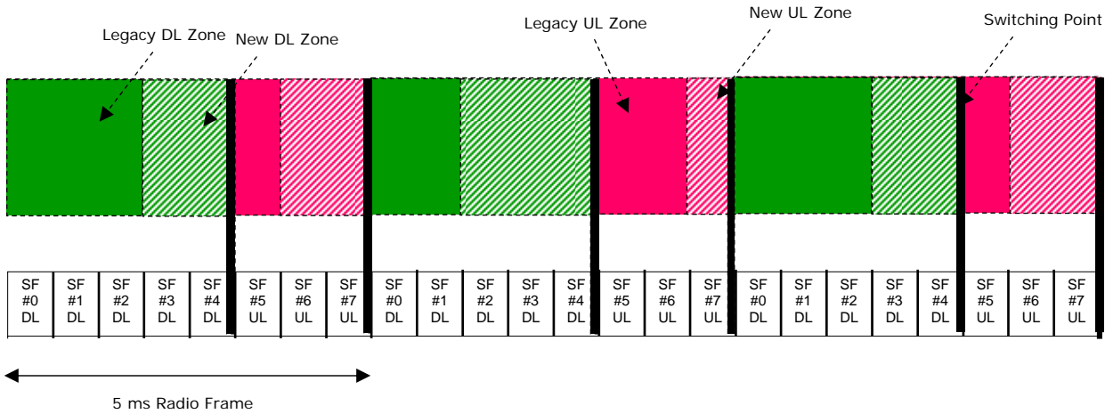
Figure 13 Figure 11.4-5: Time zones in TDD mode
