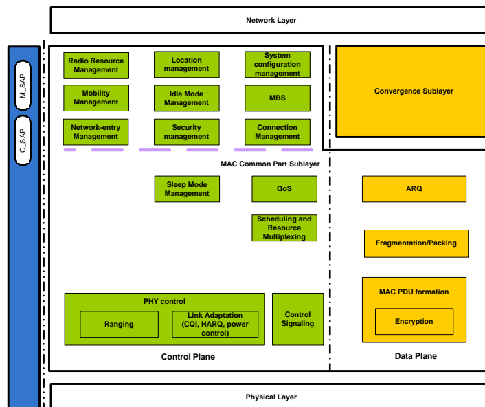
15 16 Figure 14 The IEEE 802.16e protocol architecture 17
