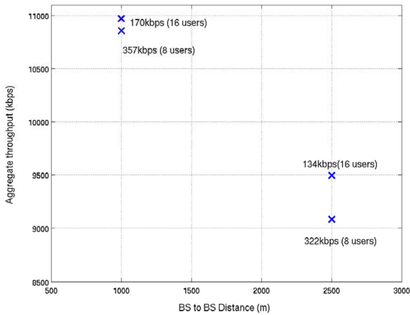
Figure 4-6 Edge user throughput vs. sector throughput and site-to-site distance for a 4x4 MIMO system with 802.20 fairness scheduling
