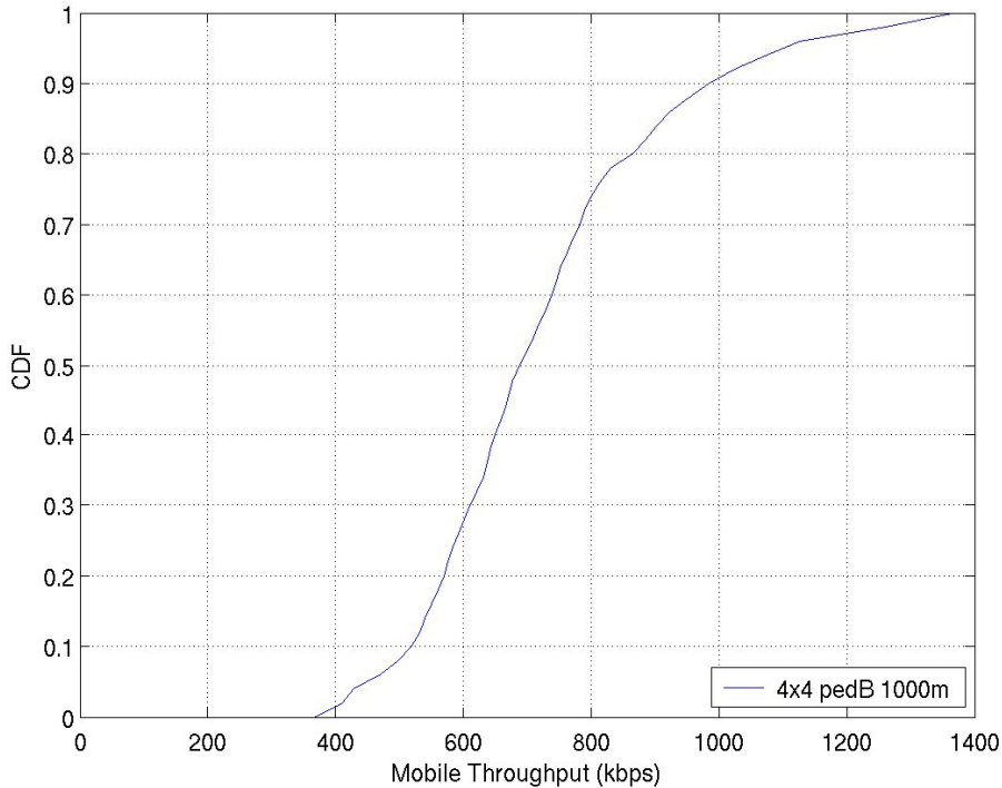
Figure 4-7 CDF of mobile throughput (1000m, 8 users/sector)
