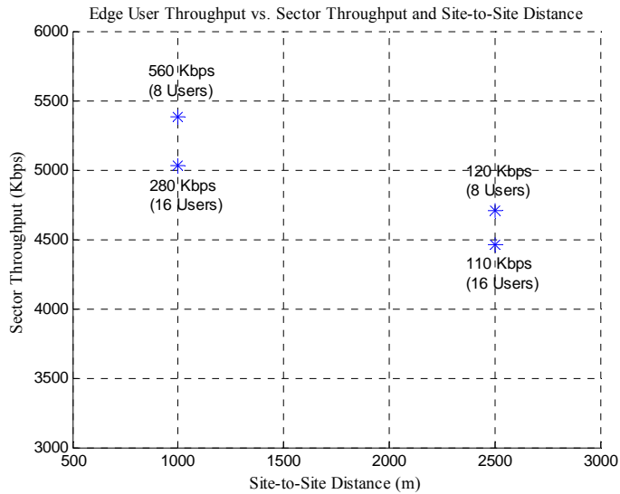
Figure 4-10 Edge user throughput vs. sector throughput and site-to-site distance
