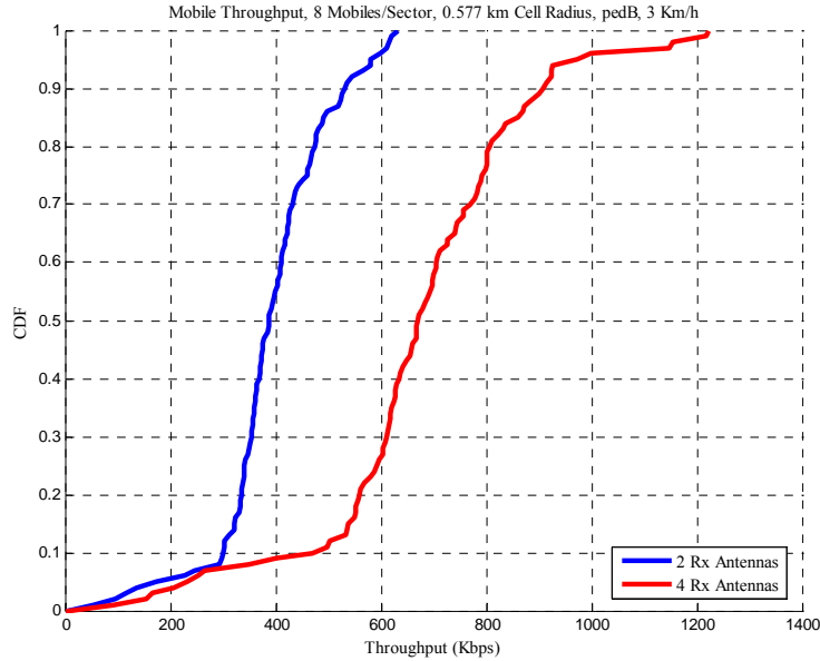
Figure 4-9 User throughput CDF for 1000m site-to-site distance and 8 users/sector, with EGoS fairness
