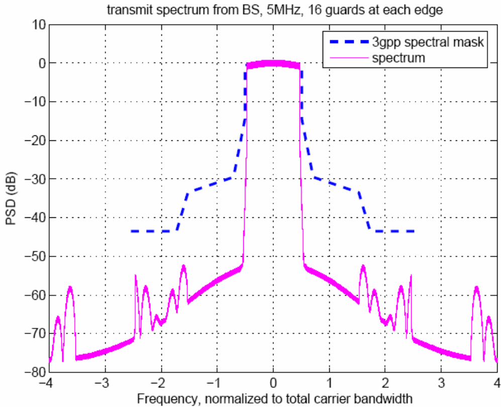
Figure 3-9 Forward link transmit spectrum
