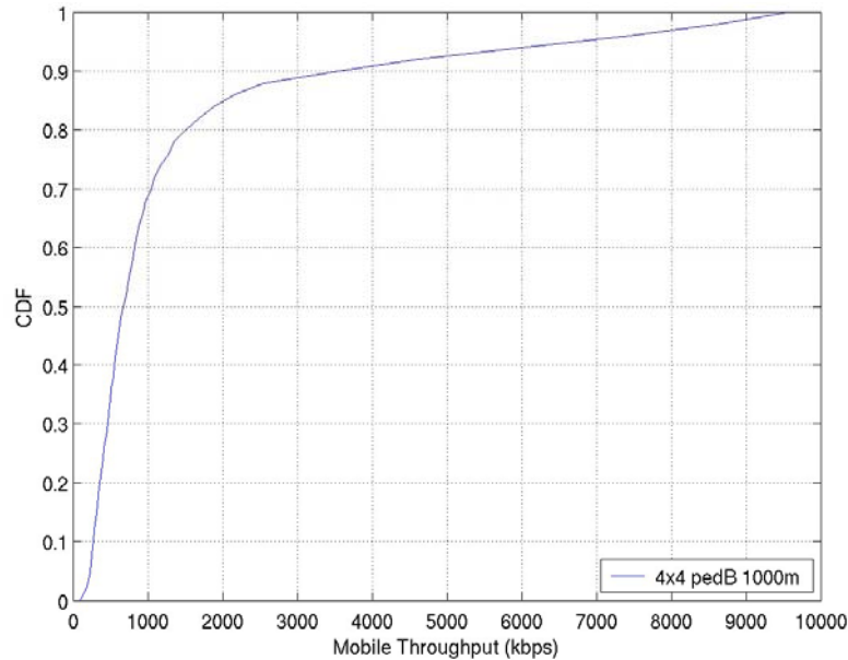
Figure 4-5 CDF of mobile throughput (1000m, 8 users/sector)
