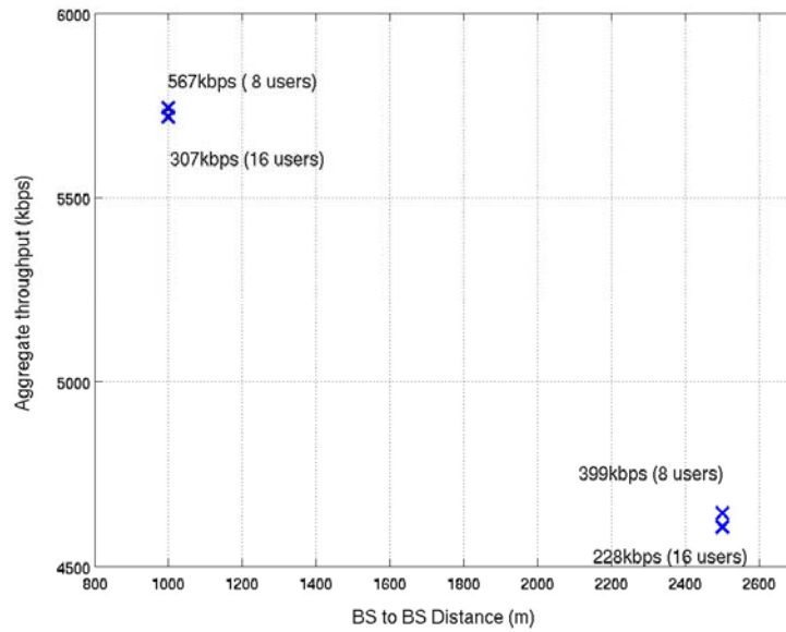
Figure 4-8 Edge user throughput vs. sector throughput and site-to-site distance for a 4x4 MIMO system with EGoS fairness scheduling
