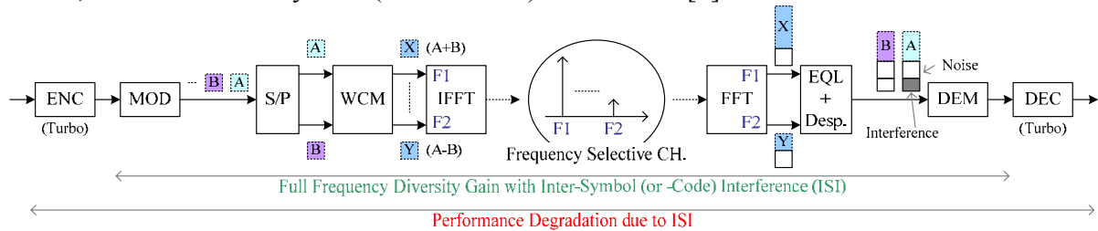
Figure 3: OFDM with Walsh code-multiplexing.
