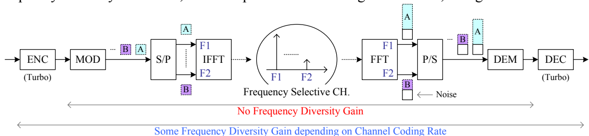
Figure 2: Normal OFDM in distributed mode.
