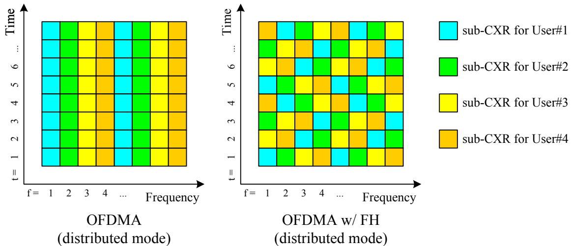
Figure 1: Distributed mode in OFDMA
