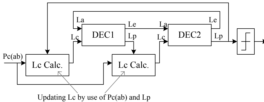
Figure 7: Twin Turbo Decoder.
