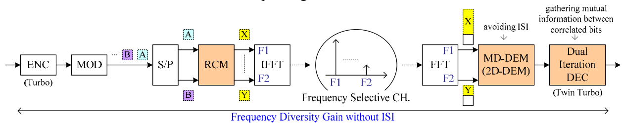
Figure 4: Rotational OFDM (R-OFDM) in distributed mode.
