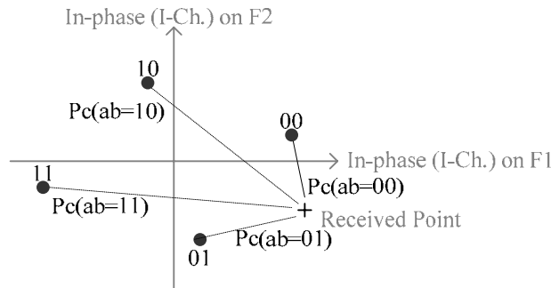
Figure 6: Signal Constellation and the Symbol Likelihood at Receiver Side.
