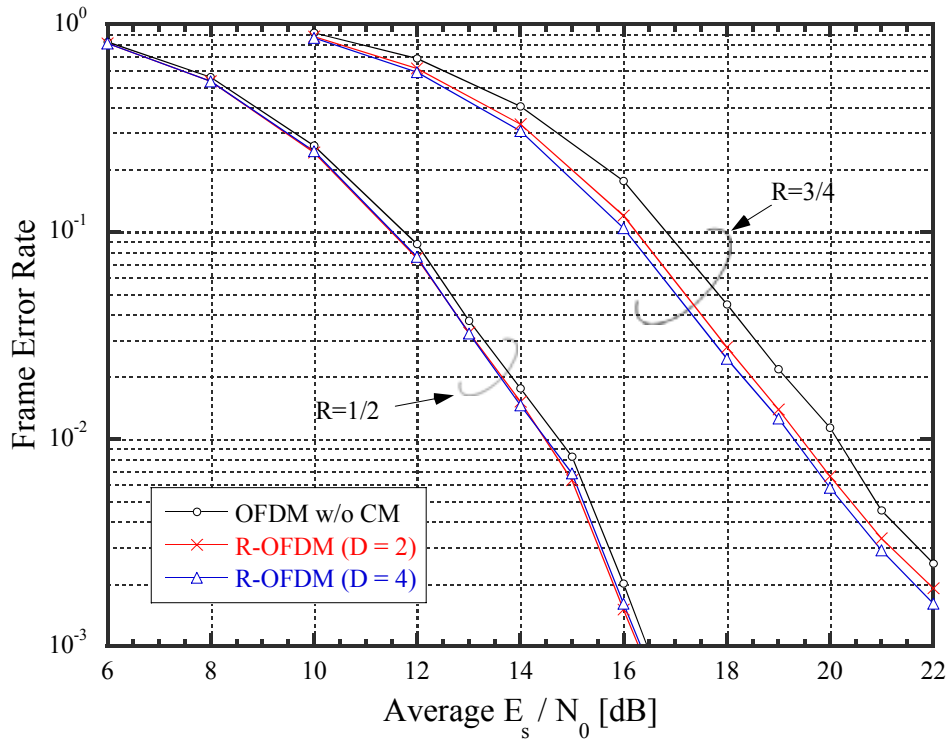
Figure 10: Frame Error Rates (16QAM in Pedestrian B channel).
