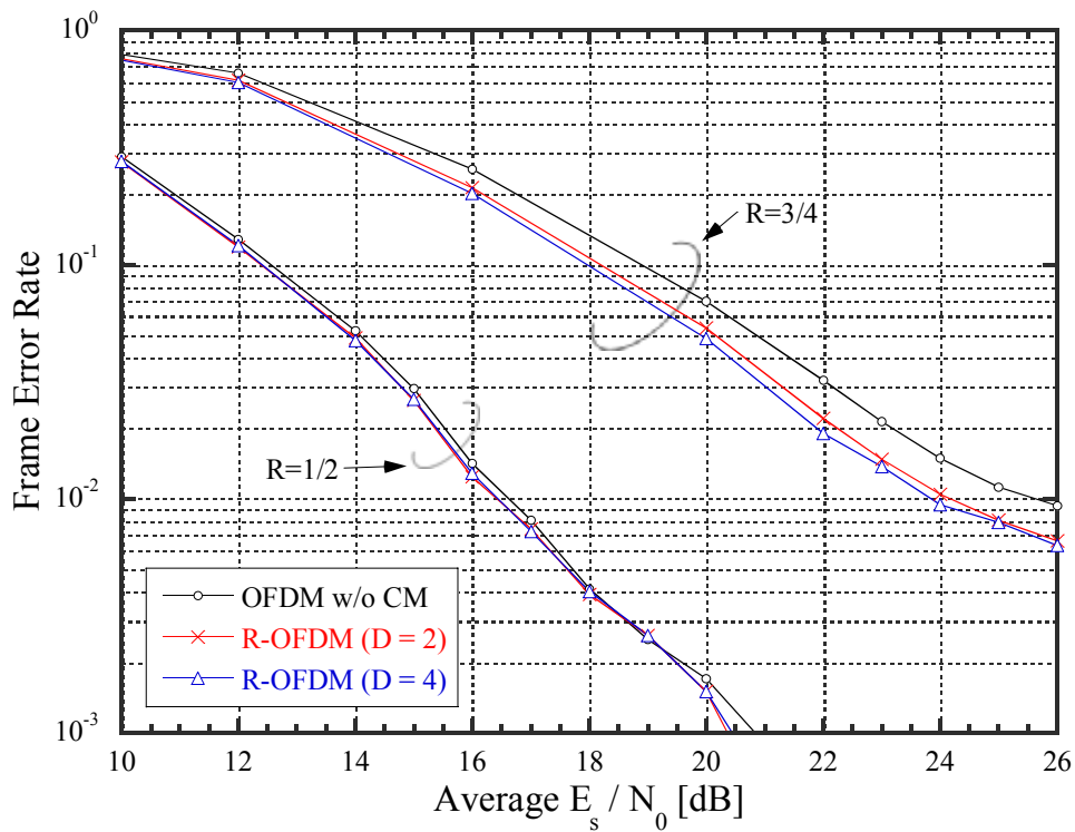
Figure 11: Frame Error Rates (16QAM in Vehicular B channel).
