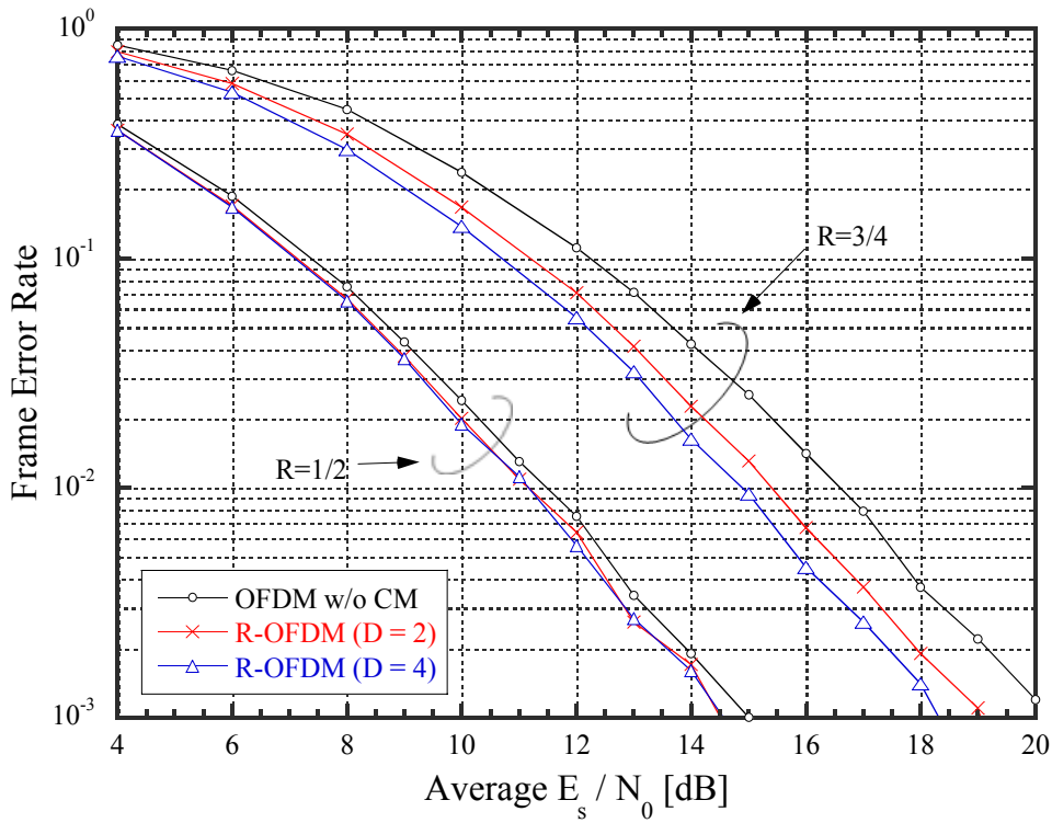
Figure 9: Frame Error Rates (QPSK in Vehicular B channel).
