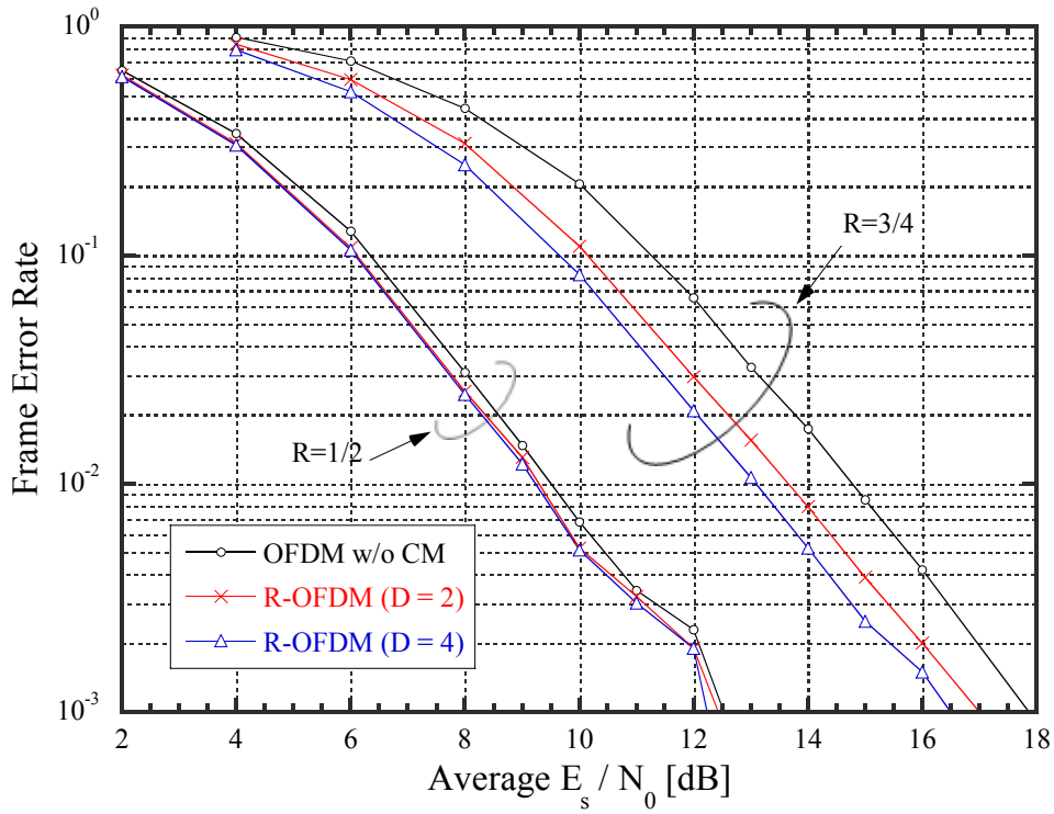
Figure 8: Frame Error Rates (QPSK in Pedestrian B channel).
