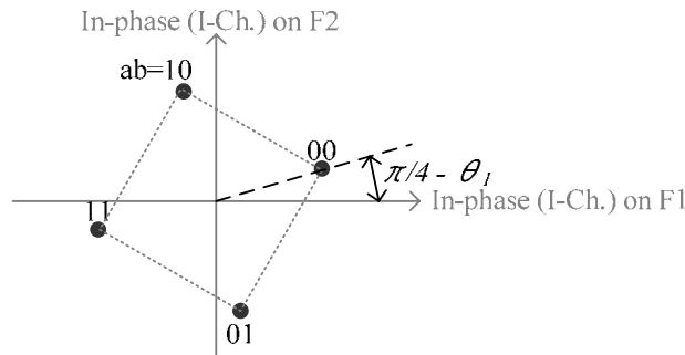
Figure 5: Signal Constellation at Transmitter Side.
