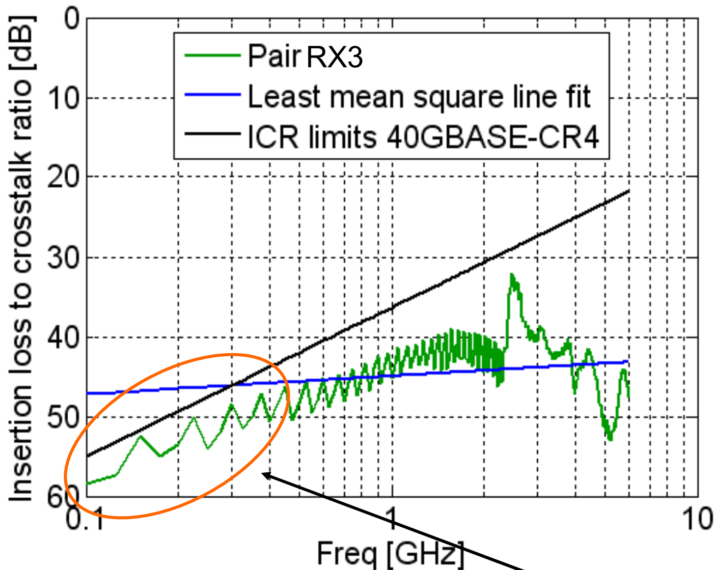
Insertion loss to crosstalk ratio
