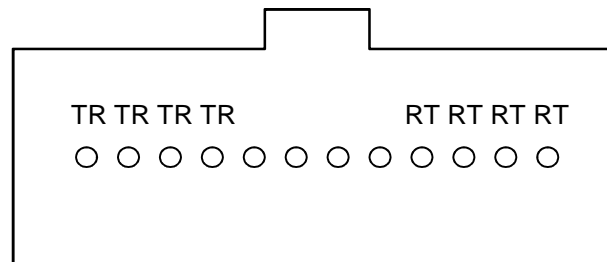
Figure 1xx-d—Optical lane assignments for 400GBASE-SR4.2
