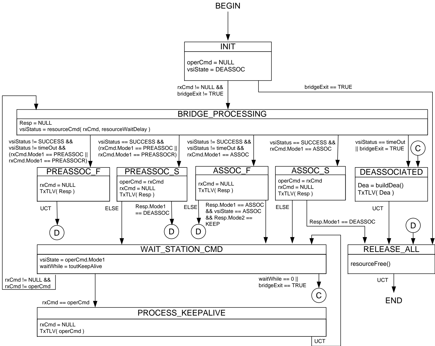
Old Bridge State Machine
