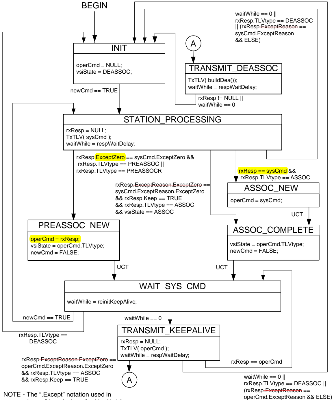
Figure 41-8—Station VDP state machine
