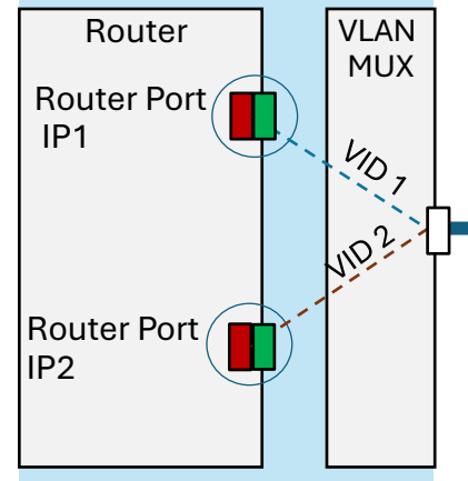
Router Subinterfaces
