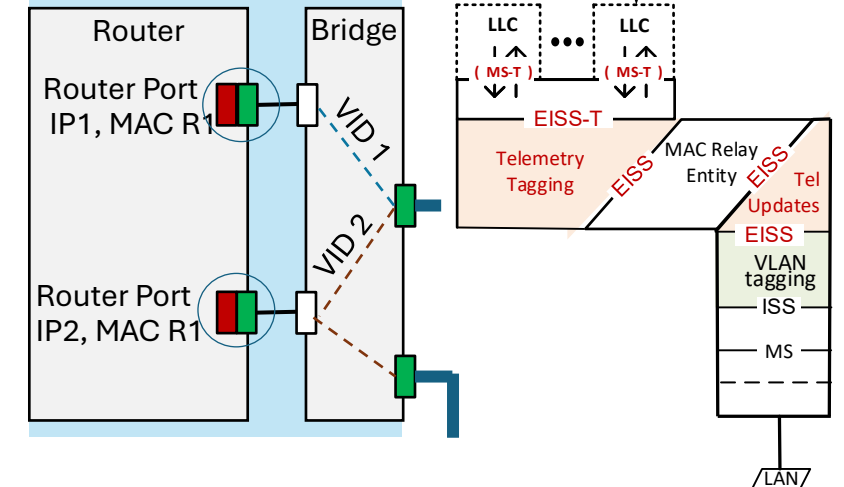
Router Switched Virtual Interfaces (SVIs)
