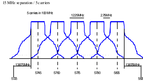
Figure 120, OFDM PHY Frequency Channel Plan
