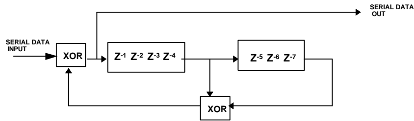
Figure 112, Data Scrambler
