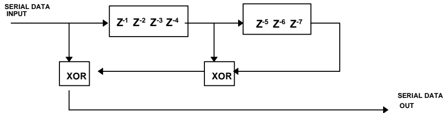
Figure 113, Data Descrambler
