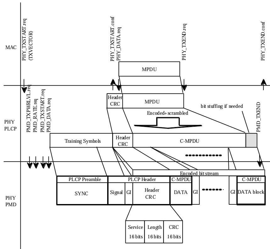
Figure 114, PLCP Transmit Procedure
