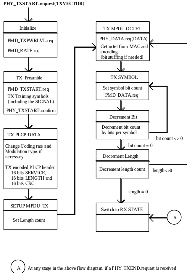
Figure 115, PLCP Transmit State Machine
