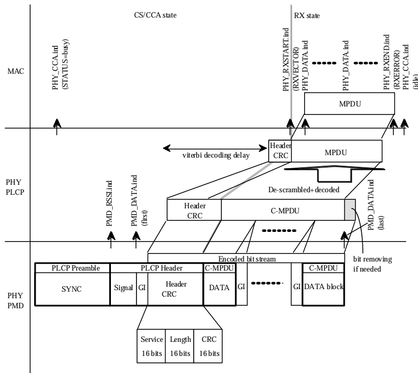
Figure 116, PLCP Receive Procedure
