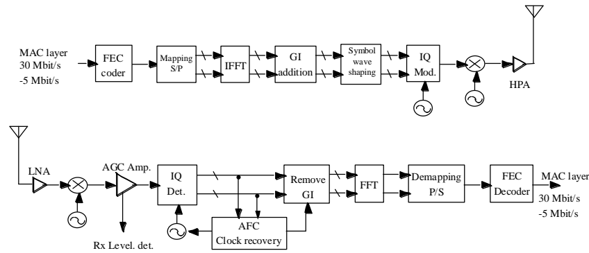
Figure 119, An Example of Transmitter and Receiver Block Diagram for OFDM PHY
