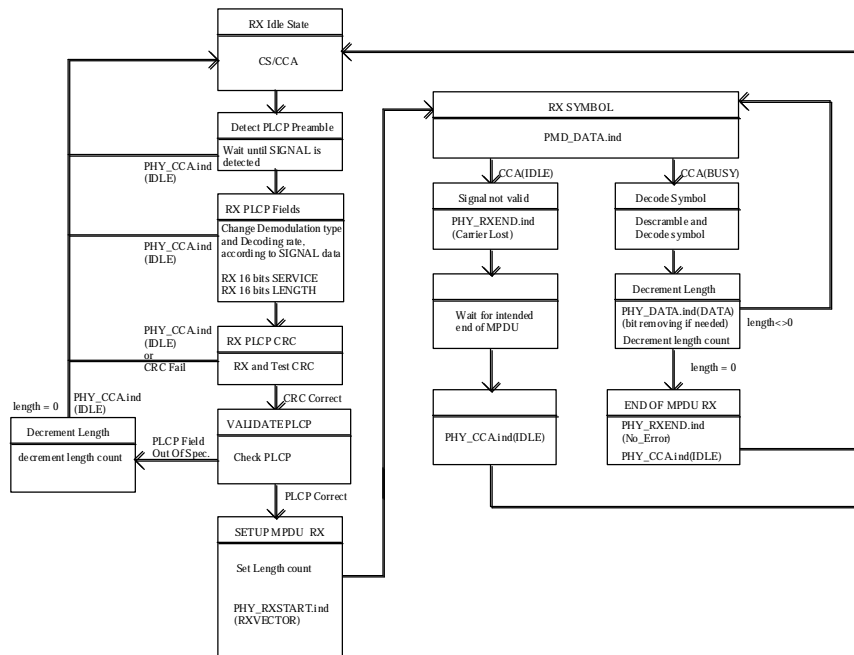
Figure 117, PLCP Receive State Machine
