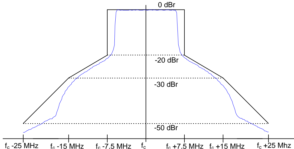
Figure 123, Transmit Spectrum Mask
