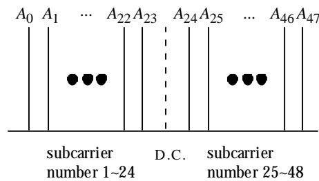
Figure 122, Subcarrier Frequency Allocation
