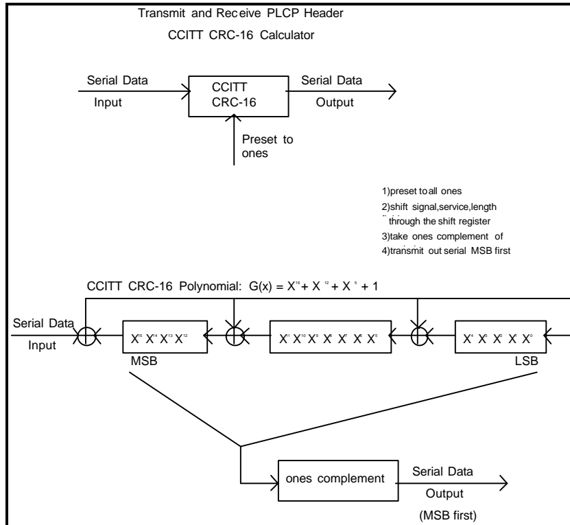
Figure 109, CCITT CRC-16 Implementation
