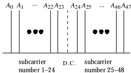
Figure 121, Subcarrier Frequency Allocation
