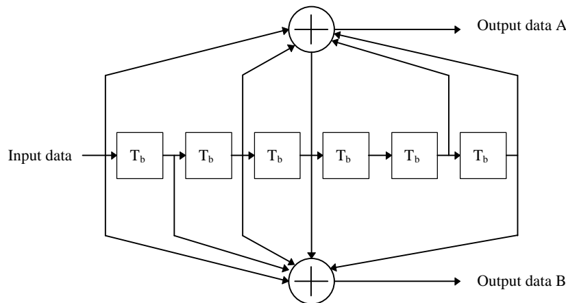
Figure 110, Convolutional Encoder
