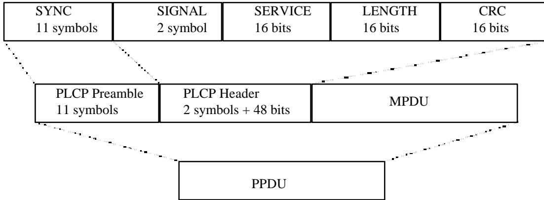
Figure 107, PLCP Frame Format
