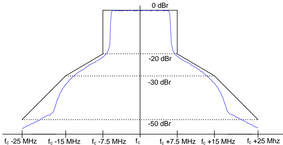
Figure 122, Transmit Spectrum Mask
