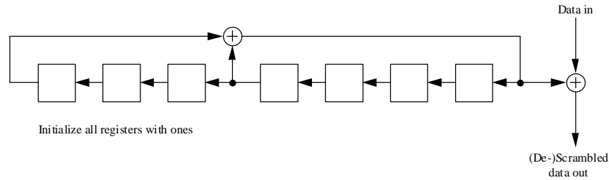
Figure 112, Data Scrambler
