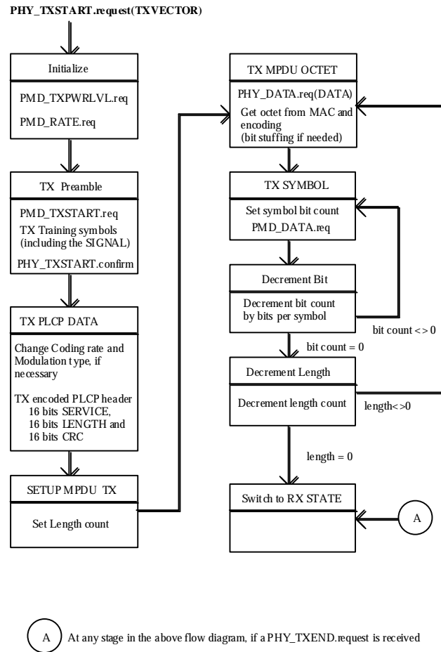
Figure 114, PLCP Transmit State Machine
