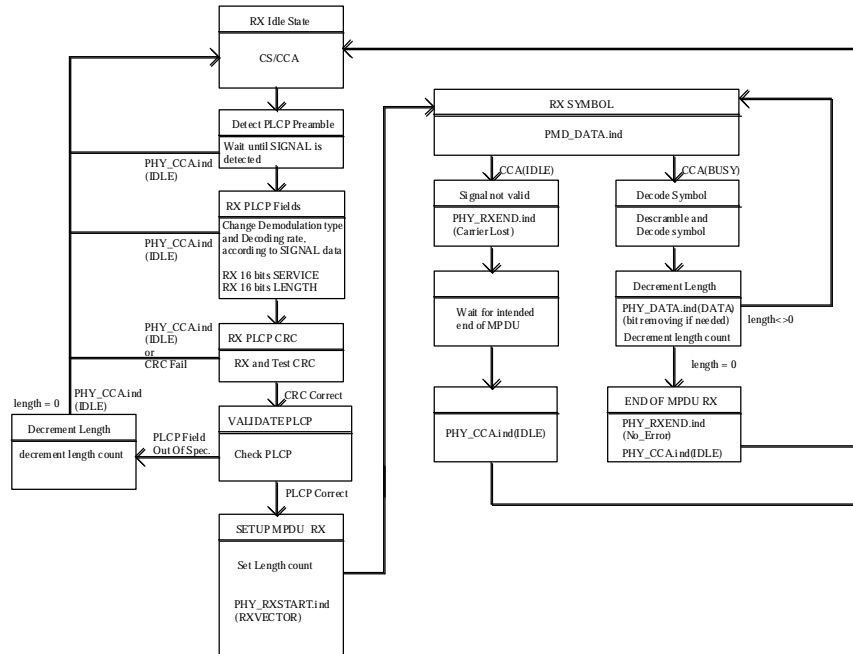
Figure 116, PLCP Receive State Machine
