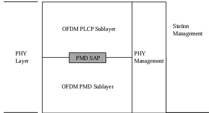
Figure 117, PMD Layer Reference Model
