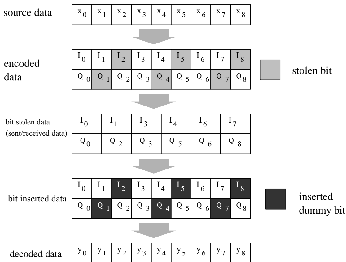
Figure 111, An example of bit-stealing and bit-insertion procedure (r=3/4)
