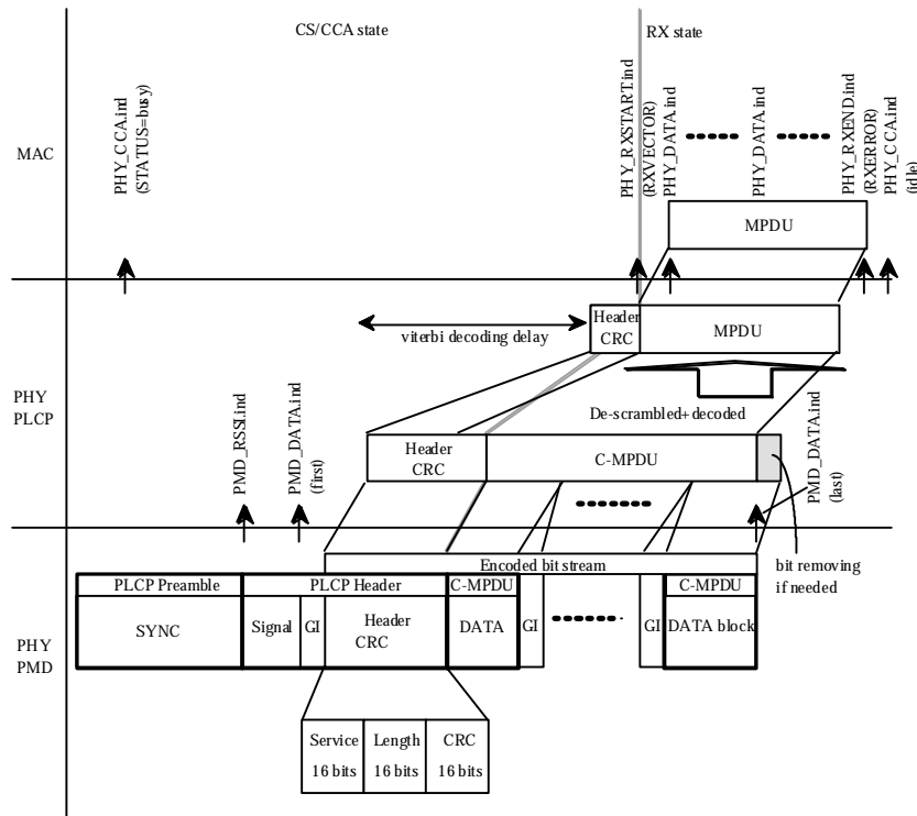
Figure 115, PLCP Receive Procedure
