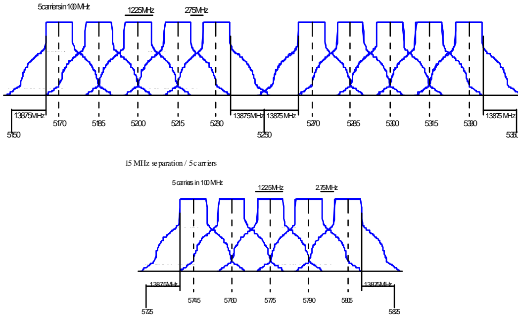
Figure 119, OFDM PHY Frequency Channel Plan
