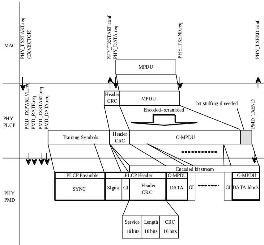
Figure 113, PLCP Transmit Procedure
