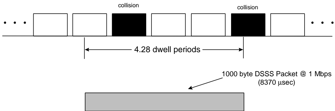
Figure 3.0-2 Increasing Hop Rate Increases Probability of Collision (FHSS System @ 512 hops/s)
