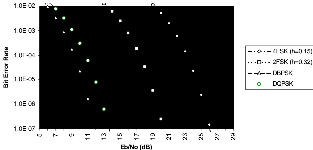
Figure 2.0-1 Eb/No vs. BER for FSK and PSK Waveforms
