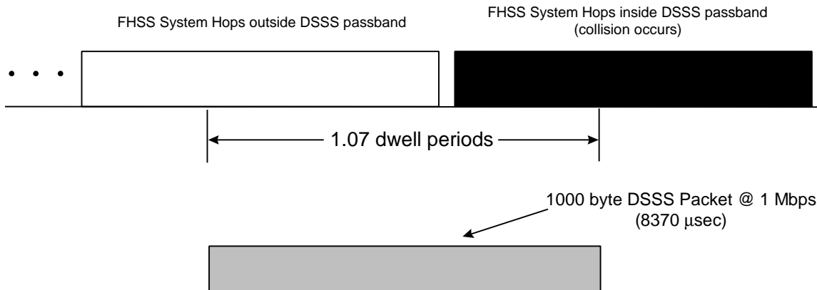
Figure 3.0-1 Probability of Collision Depends on Hop Rate (FHSS System @ 128 hops/s)
