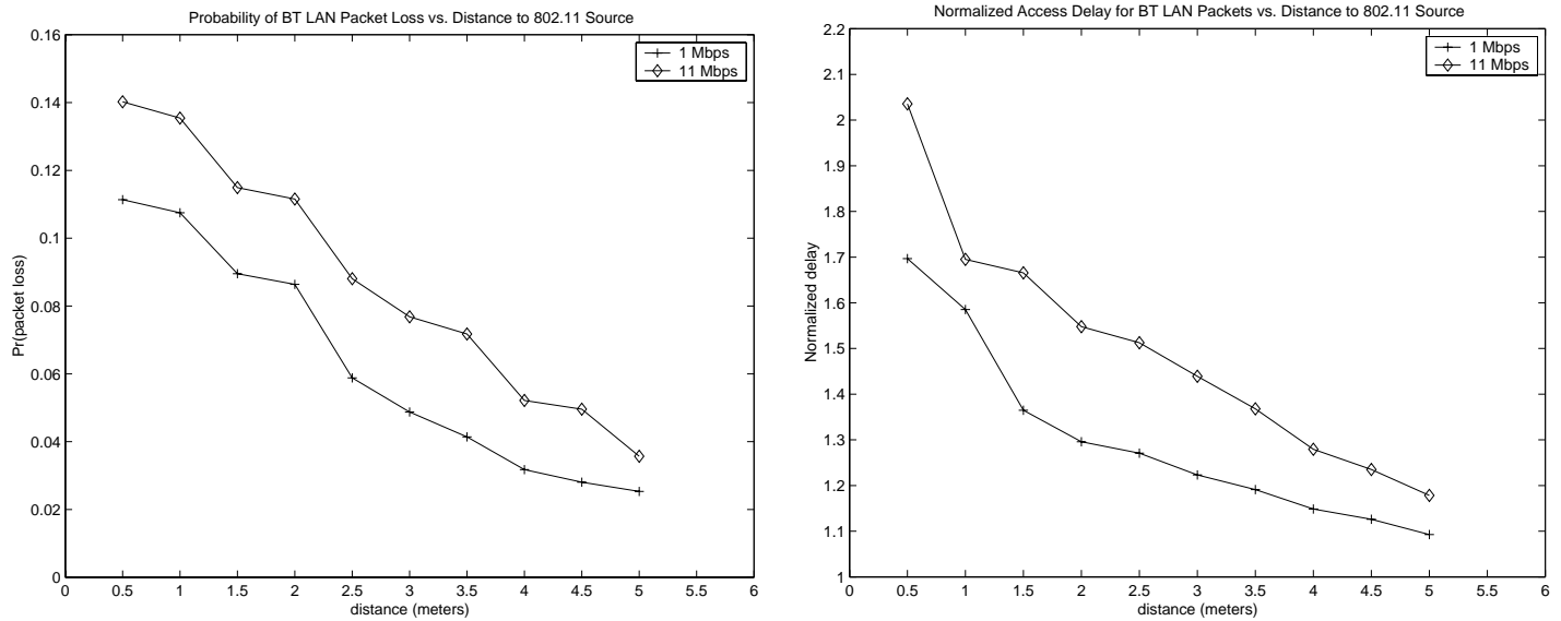
Fig. 5. (a) (b) Experiment 2. Bluetooth data packets with 802.11 interference. (a) Probability of packet loss. (b) Access delay.
