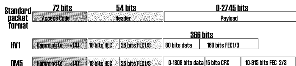
Fig. 1. Bluetooth Packet Format
