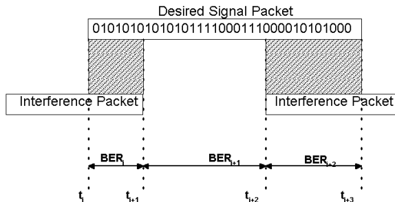
Fig. 2. Packet Collision and Placement of Errors
