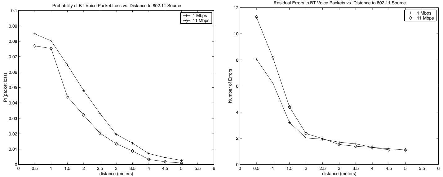
Fig. 4. (a) (b) Experiment 1. Bluetooth voice packets with 802.11 interference. (a) Probability of packet loss. (b) Residual errors.
