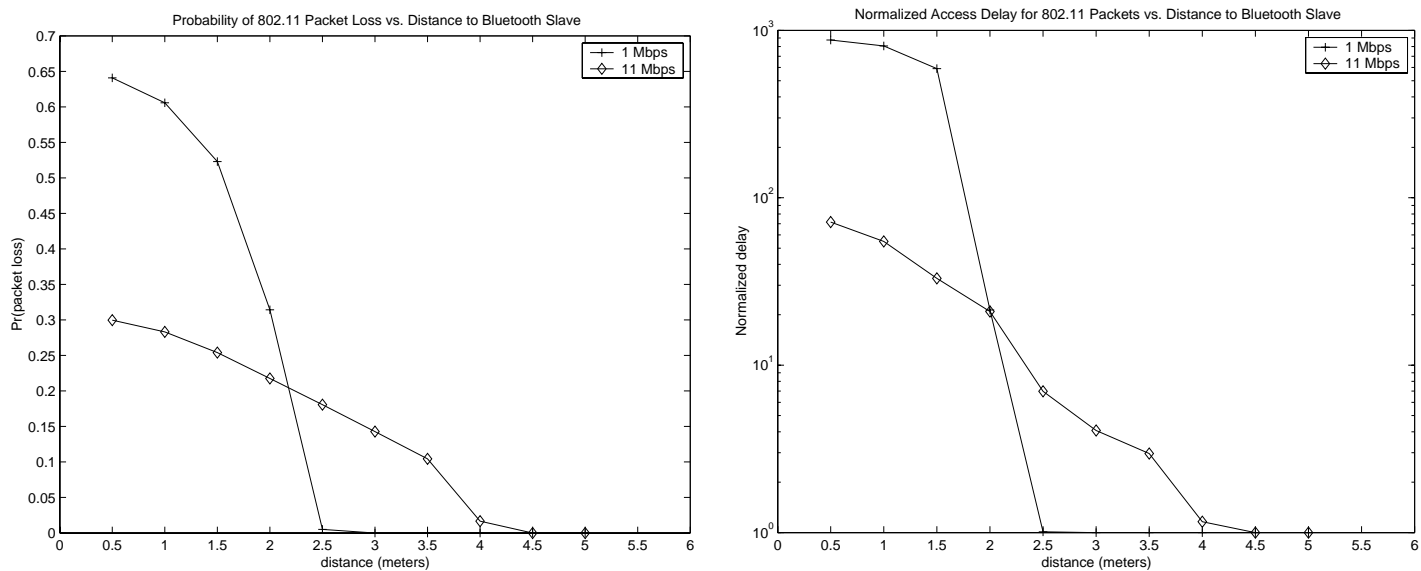
Fig. 6. (a) (b) Experiment 3. 802.11 packets with Bluetooth voice packets as interference. (a) Probability of packet loss. (b) Delay.
