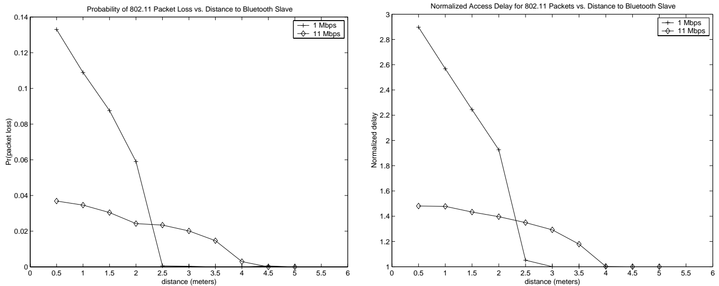
Fig. 7. (a) (b) Experiment 4. 802.11 packets with Bluetooth LAN packets as interference. (a) Probability of packet loss. (b) Delay.
