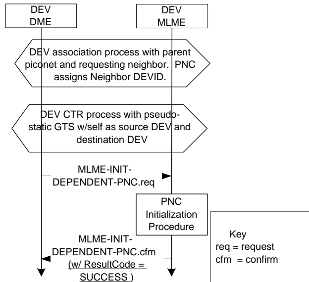
Figure 5—MSC for the initiating of a neighbor piconet.
