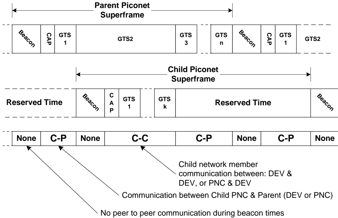
Figure 2—Parent piconet and child piconet superframe relationship
