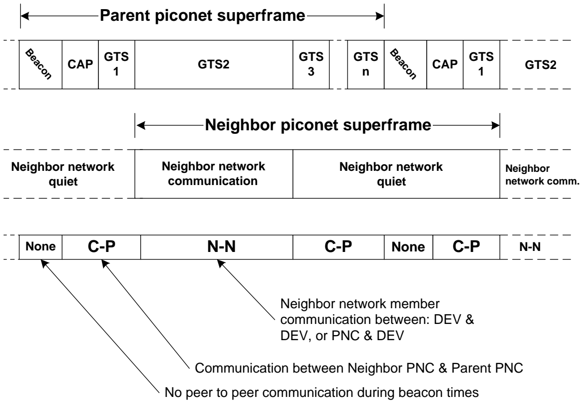
Figure 4—Parent piconet and neighbor piconet superframe relationship
