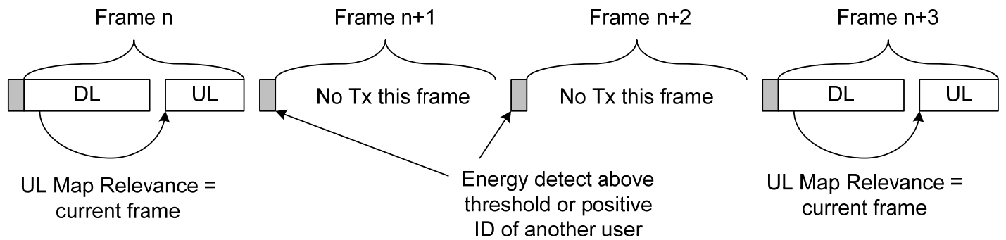
Figure x4: Listen-Before Talk
