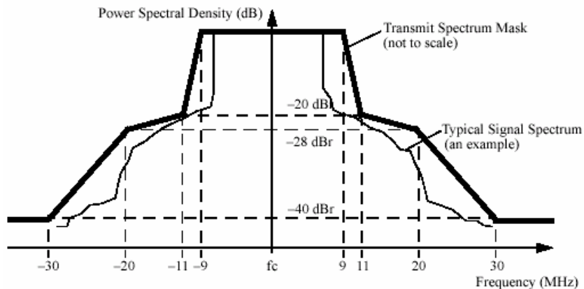
Figure 124—Transmit spectrum mask
