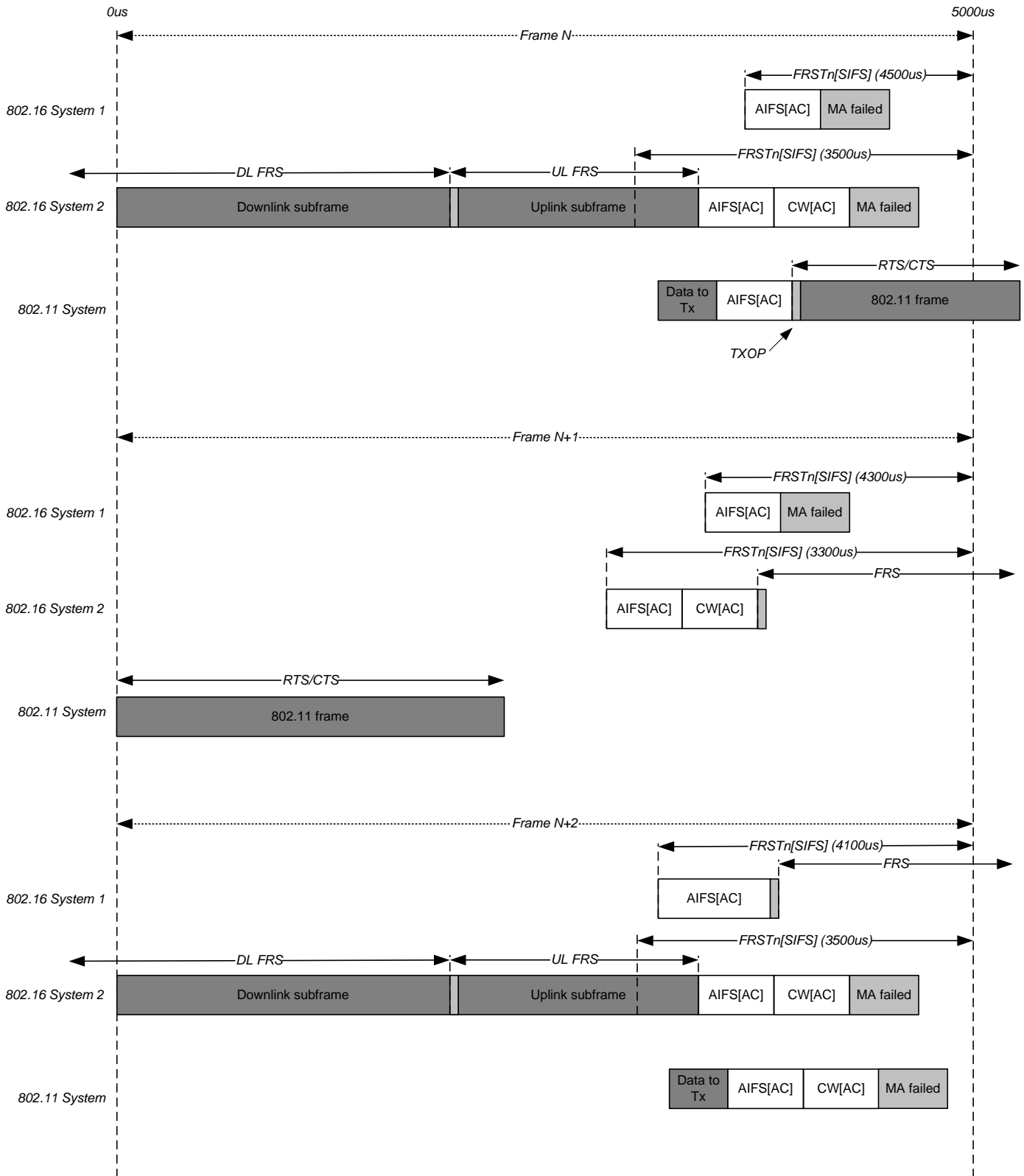
Figure h200803-01 – A detailed example of 2 802.16 and 1 802.11 systems sharing the medium over 3 frame intervals. 802.16 System 2 has Frame N, 802.11 uses Frame N+1, and 802.16 System 2 claims Frame N+2. 802.16 System 1 claims Frame N+3.
