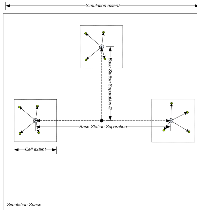
Figure 17 Spatially distributed simulation configuration: 3 systems.
