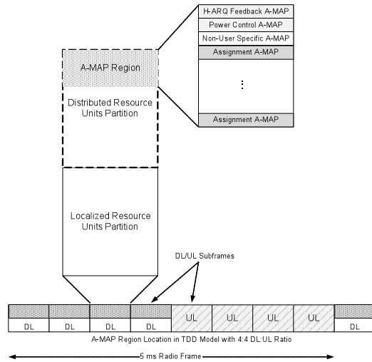
Figure 8: A-MAP Location and Structure (Example)
