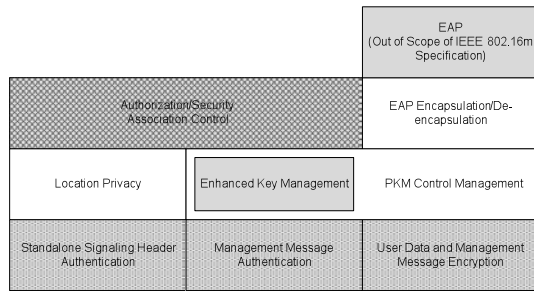
Figure 17: Functional Blocks of WirelessMAN-Advanced Security Architecture
