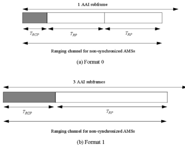
Figure 10: Ranging Channel Structure for Non-synchronized Access
