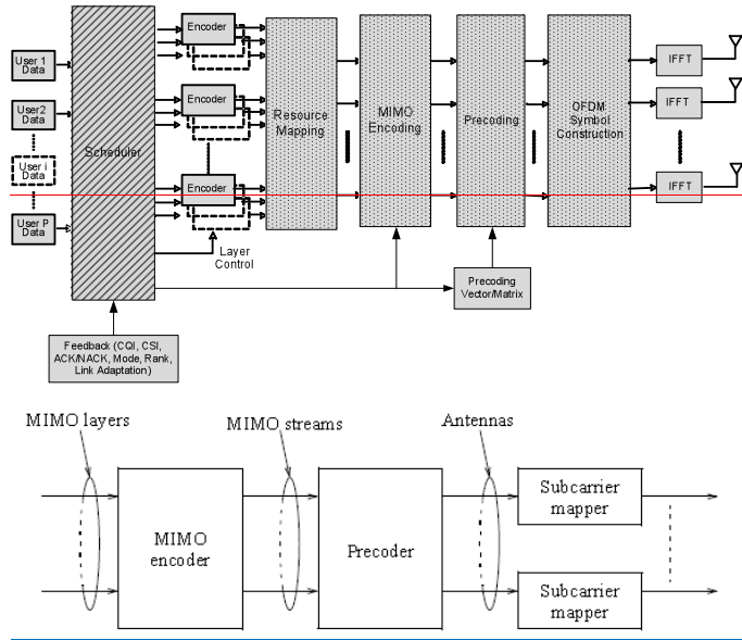
Figure 12: Illustration of Downlink MIMO Structure
