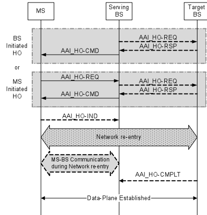
Figure 16: WirelessMAN-Advanced Handover Procedure
