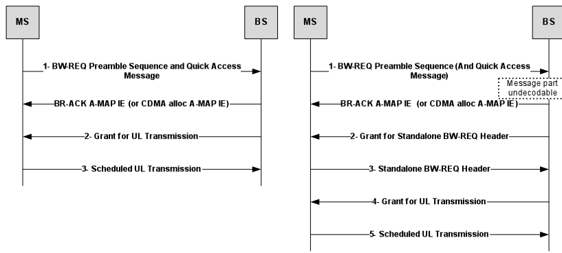
Figure 9: Bandwidth Request Procedure
