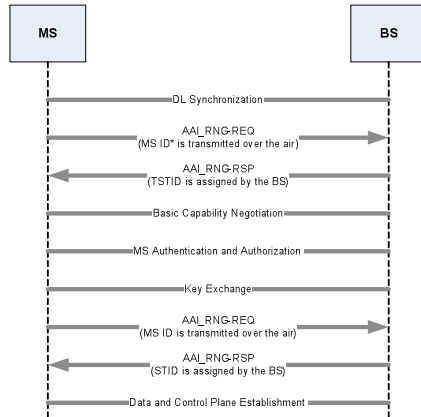
12 13 Figure 14: Network Entry Procedures
