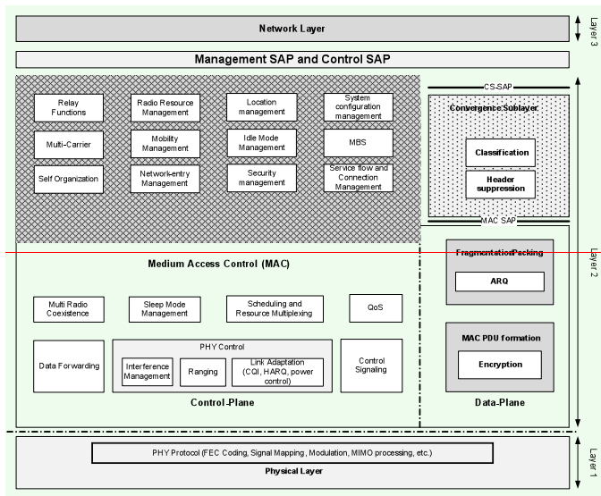
22 23 Figure 1: IEEE WirelessMAN-Advanced Protocol Stack
