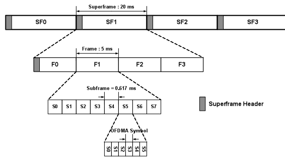
Figure 3: Basic Frame Structure
