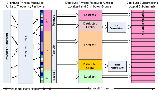
Figure 4: Illustration of the Downlink/Uplink Subcarrier to Resource Unit Mapping where P_i denotes the i th Frequency Partition
