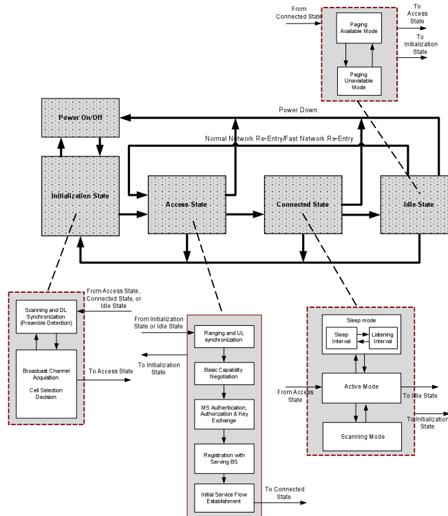
Figure 2: Mobile Station State Diagram
