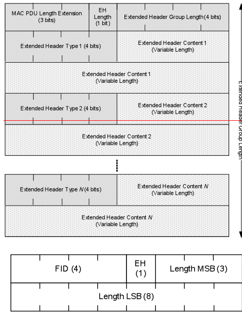
Figure 15: Structure of the WirelessMAN-Advanced Generic MAC Headers
