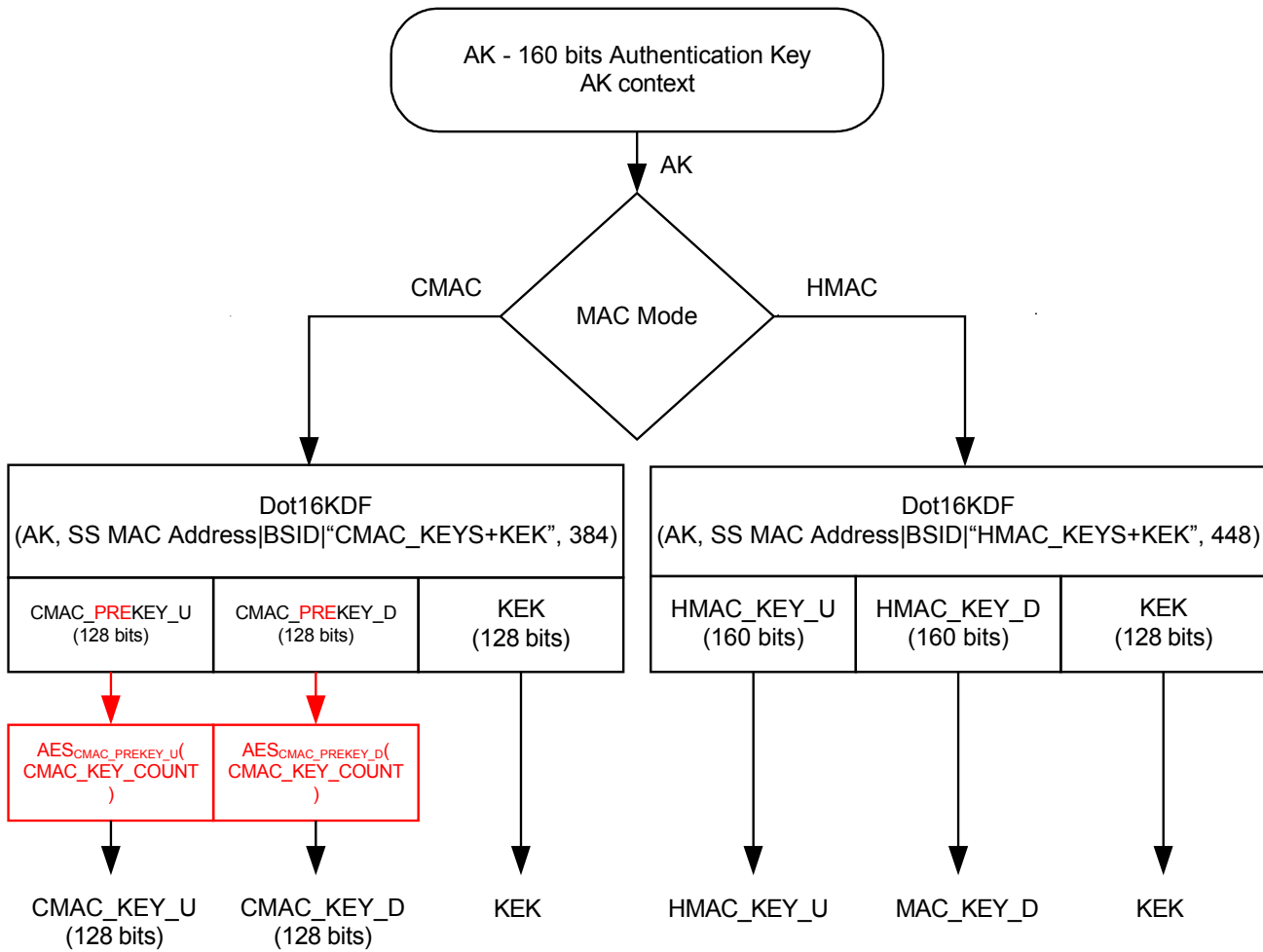
Figure 130o—HMAC/CMAC/KEK derivation from AK
