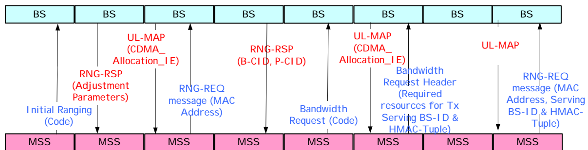
Figure 1 Handover ranging procedure using the same codes for handover/initial ranging(Not optimized bandwidth allocation, allocating the resources for only initial ranging, by BS.)
