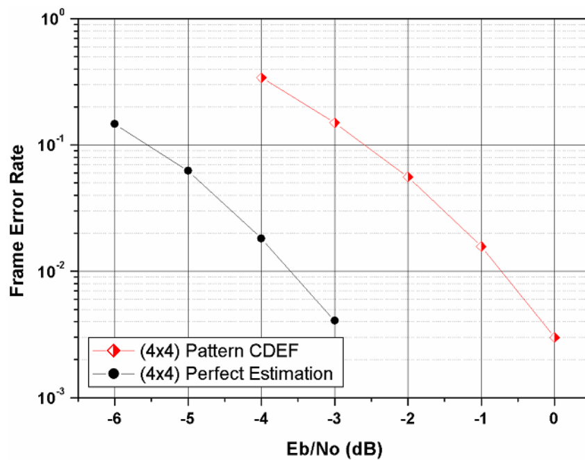
Figure 7. FER for dual MSSs with dual antennas and BS with 4 antennas (Vehicular A with 60km/h)
