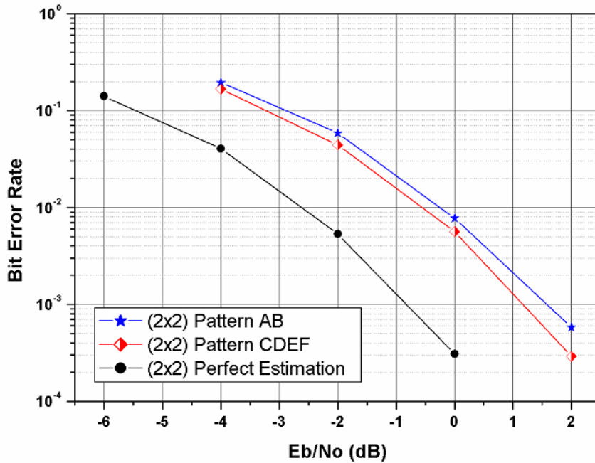
Figure 2. BER for single MSS with dual antennas and BS with dual antennas (Pedestrian B with 10km/h)
