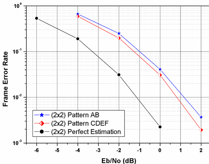
Figure 3. FER for single MSS with dual antennas and BS with dual antennas (Pedestrian B with 10km/h)
