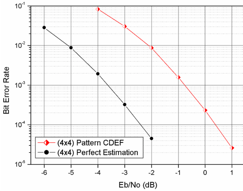
Figure 4. BER for dual MSSs with dual antennas and BS with 4 antennas (Pedestrian B with 10km/h)
