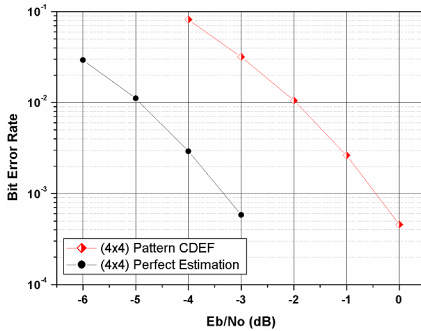
Figure 6. BER for dual MSSs with dual antennas and BS with 4 antennas (Vehicular A with 60km/h)
