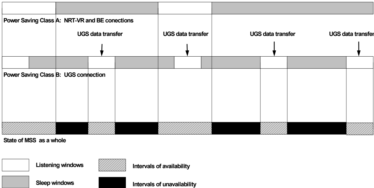
Figure NNN. Example of Sleep Mode Operations with two Power Saving Classes
