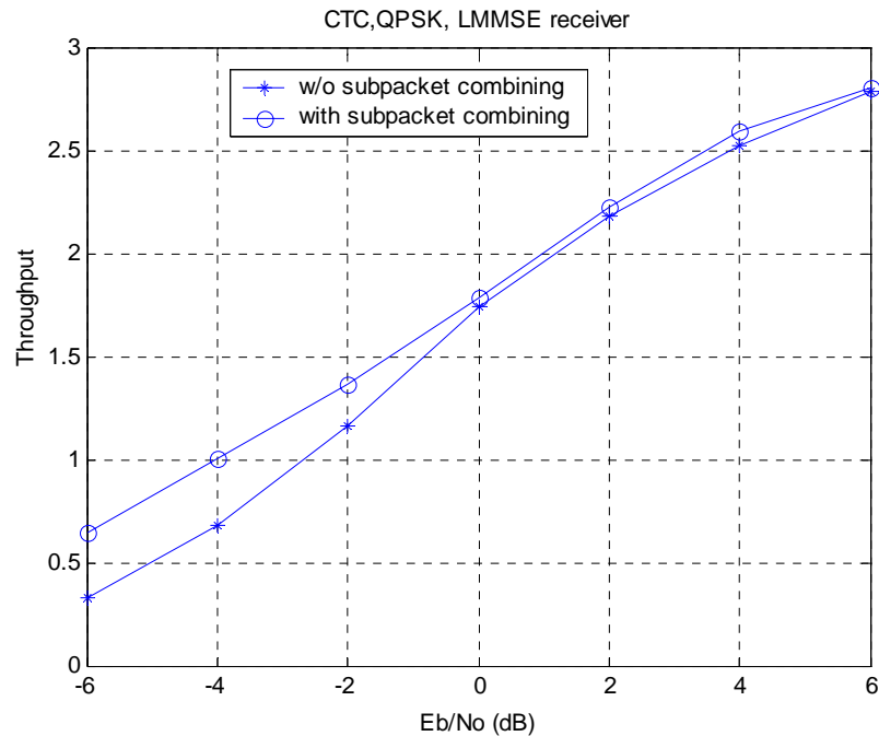
Figure 1. Throughput comparison with and without subpacket combining with matrix B.
