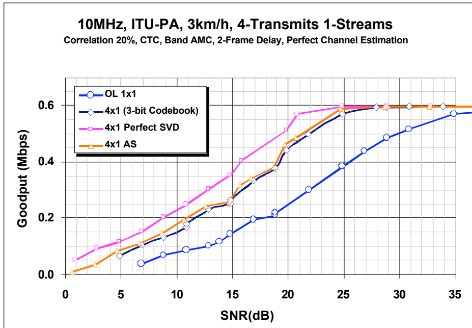
Figure 5 Comparison of AS with the 3-bit Compact Codebook Beamformer (4 transmit and 1 stream case)
