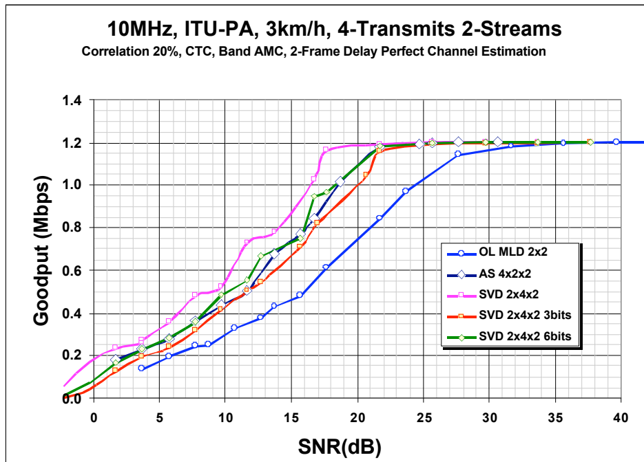
Figure 6 Comparison of AS with the 3-bit Compact Codebook Beamformer (4 transmit and 2 streams case)
