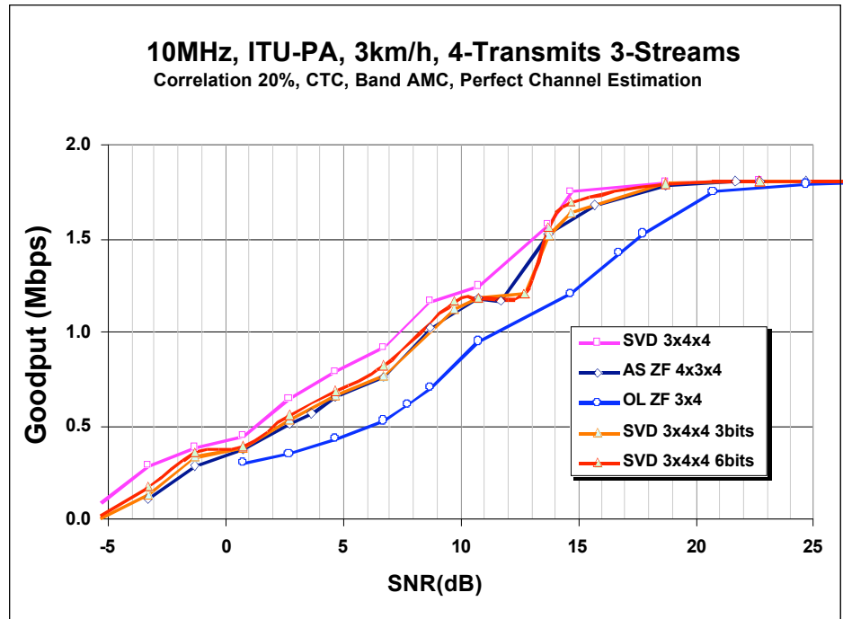
Figure 7 Comparison of AS with the 3-bit Compact Codebook Beamformer (4 transmit and 3 streams case)
