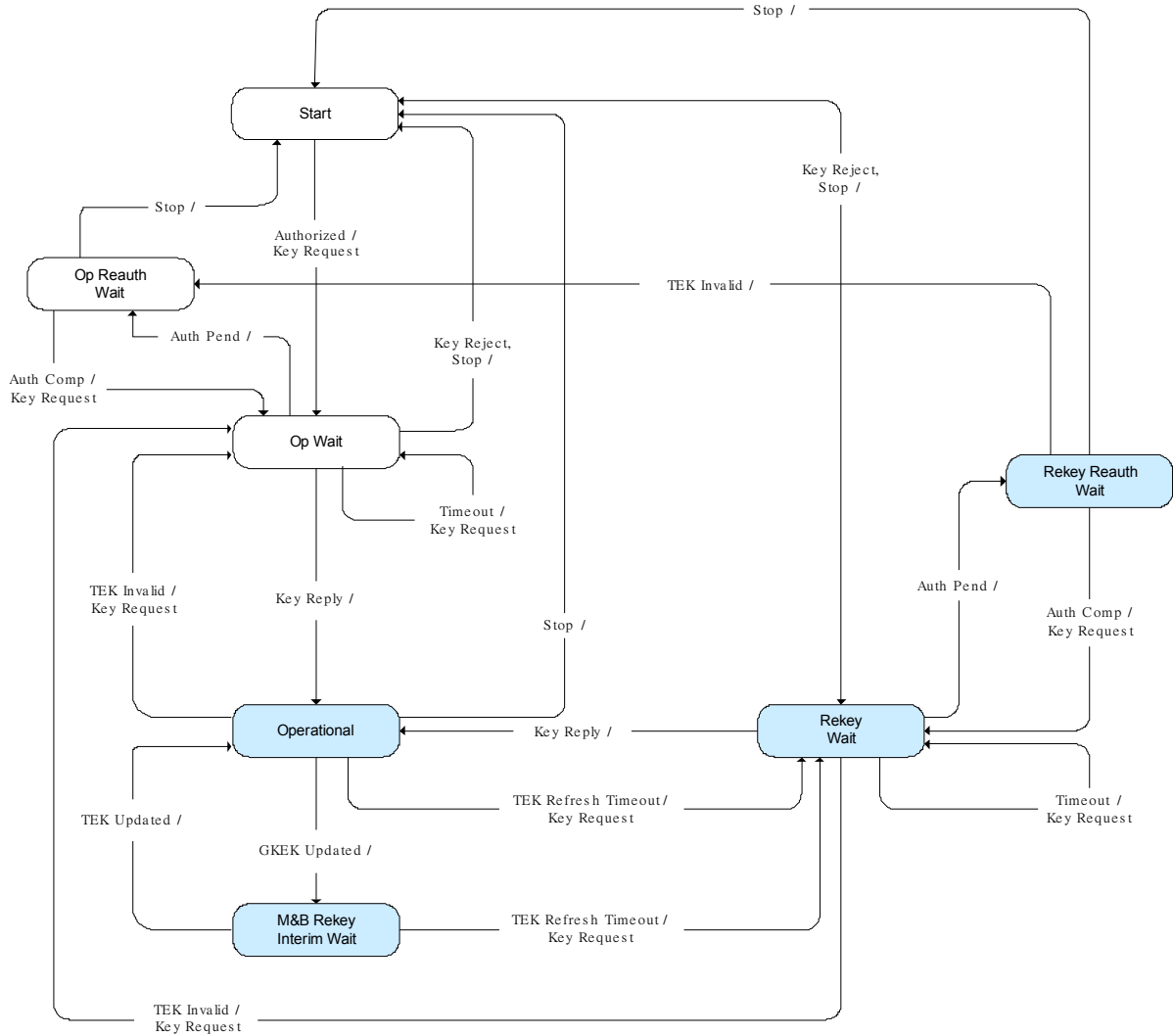
Figure 132-TEK state machine flow diagram
