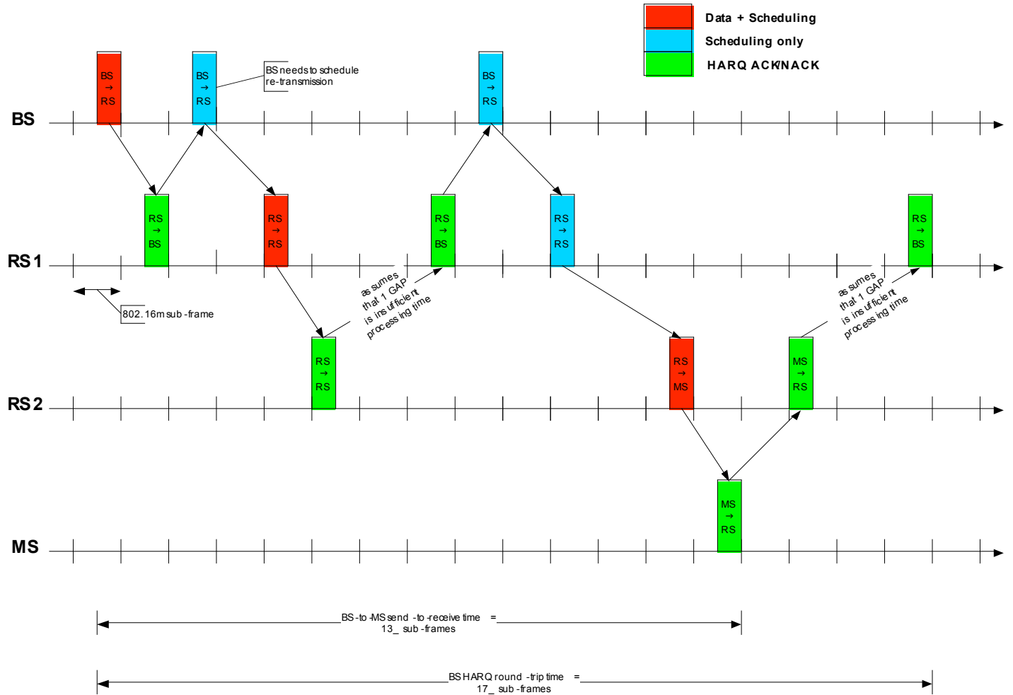
0 1 Figure 8. Timing diagram of downlink with Simple 3-hop and centralized scheduling 2 3
