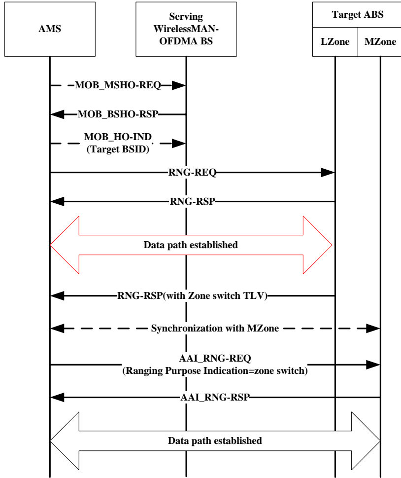
Figure 410— Handover procedure from WirelessMAN-OFDMA BS to ABS: the T-ABS instructs AMS to switch zone after completion of network reentry at LZone
