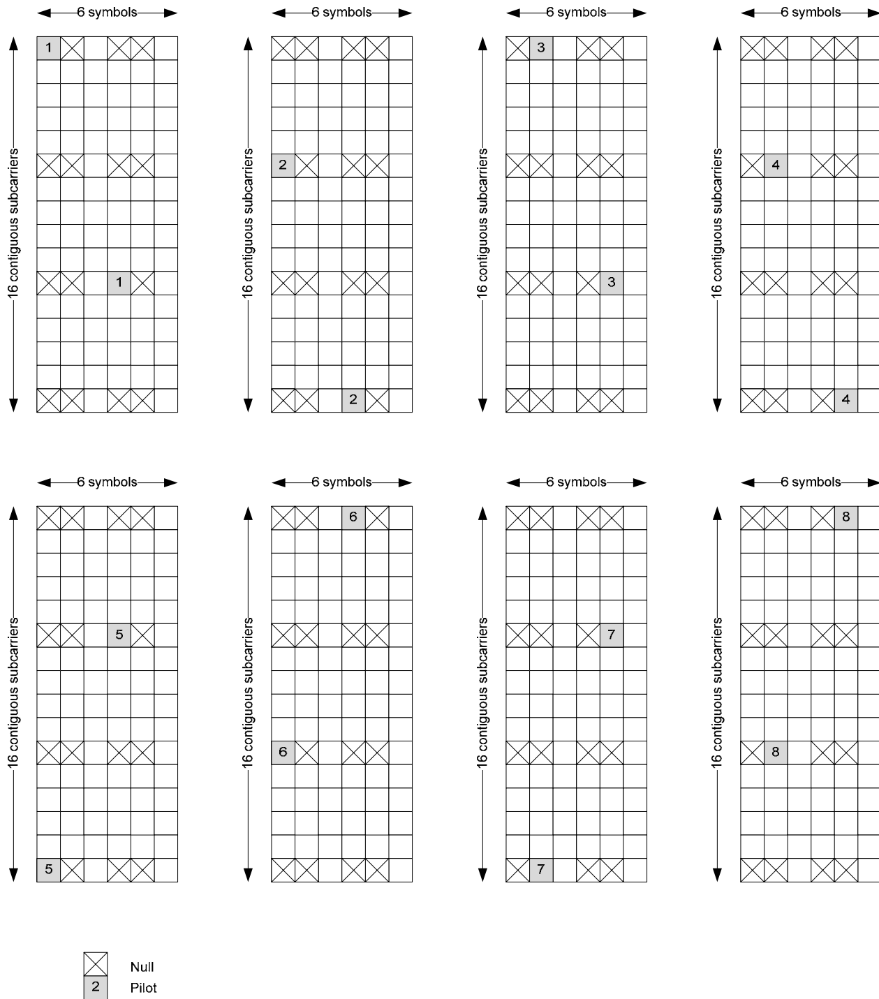
Figure 504c. Pilot patterns for 8 downlink only data streams
