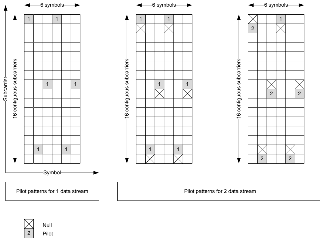
Figure 504a. Pilot patterns for 1 and 2 data streams
