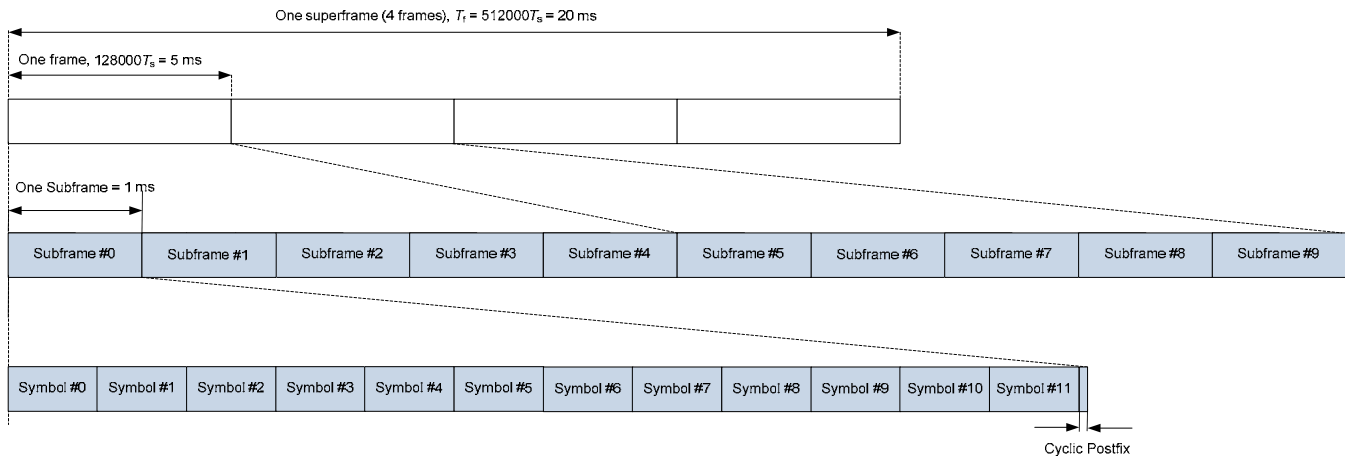
Figure 468a Basic frame structure for FDD mode
