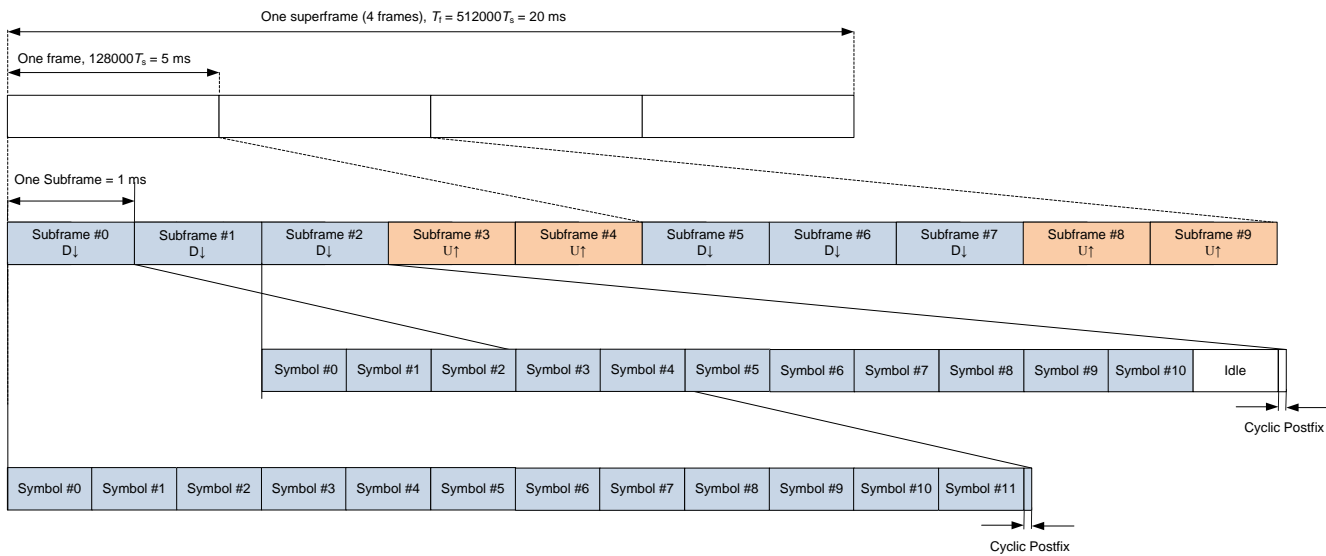
Figure 468b. Frame Structure Type for TDD mode
