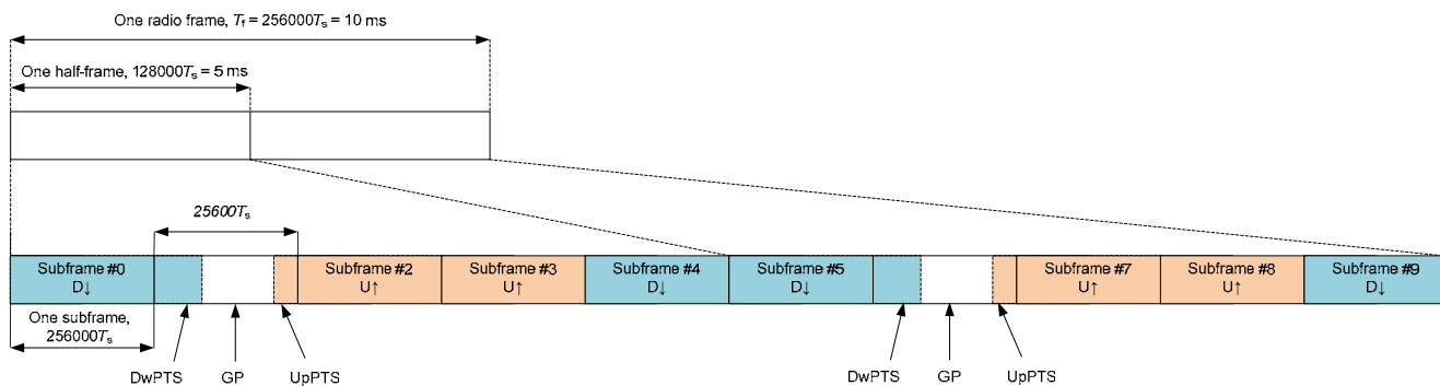
Figure 468c Frame structure with special subframe
