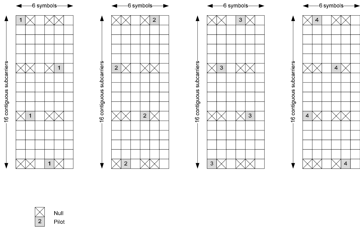
Figure 504b. Pilot patterns for 4 data streams
