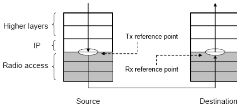
14 Figure 1-Illustration of reference points for the maximum user-plane data latency
