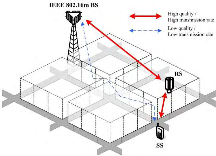
Figure 3—Deploying RS can enhance transmission rate for the SS located in shaded area or cell boundary
