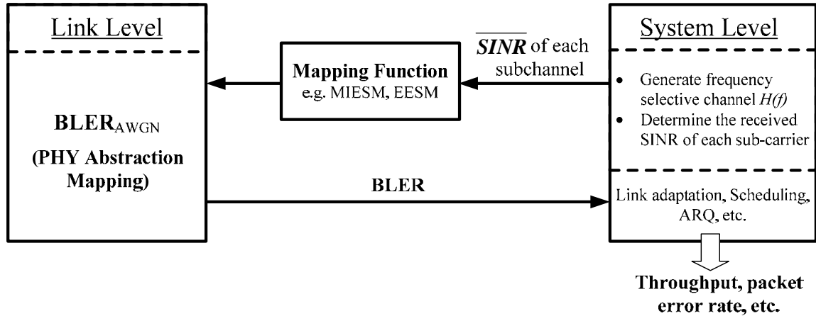
7 8 Figure 7: PHY link-to-system mapping procedure 9
