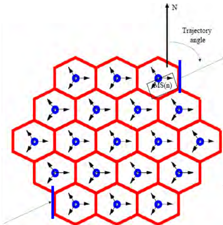
19 20 21 Figure 17: 19 cell abbreviated example of MS movement in a wrap around topology * 22
