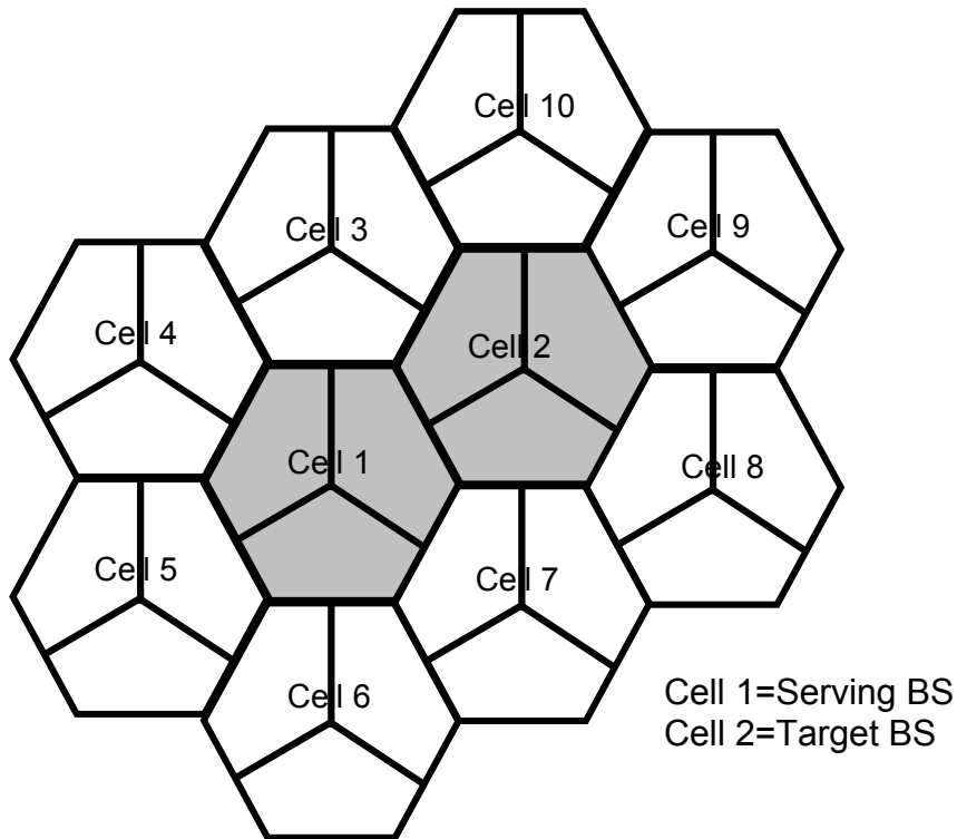
Figure 16: 10 Cell topology
