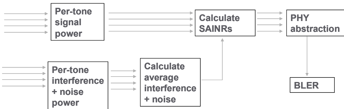
25 26 27 28 29 30 31 32 33 34 35 36 37 38 39 40 Figure 11: PHY abstraction simulation procedure for average interference knowledge
