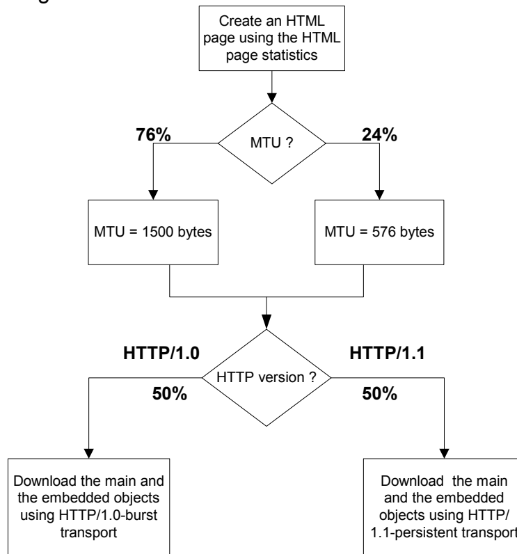
10 11 12 13 Figure 19: HTTP traffic profiles
