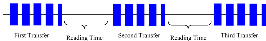
11 Figure 20: FTP traffic patterns
