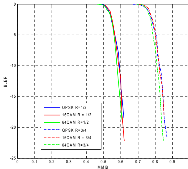
18 Figure 10: BLER ( \log_{10} scale) mappings for MMIB from AWGN performance results 19
