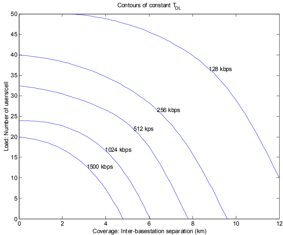
Figure 2: Contours of constant minimum service level
