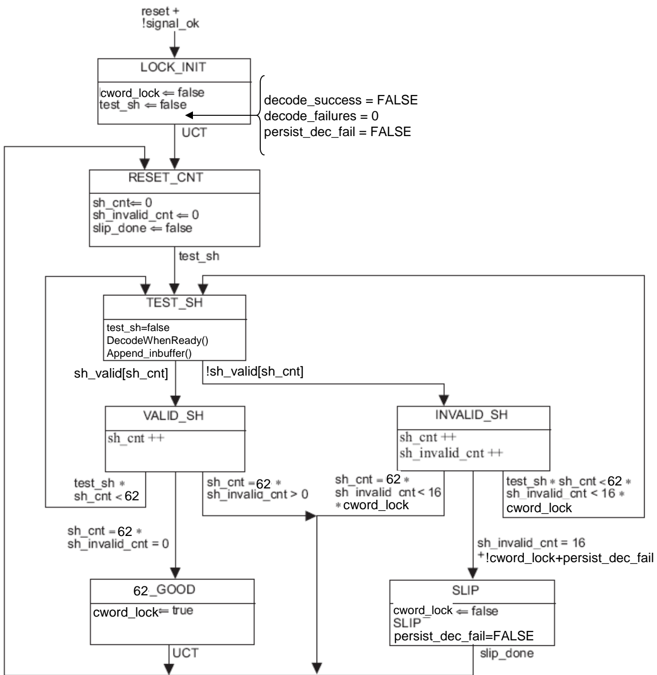
Figure 92-10—Lock state machine
