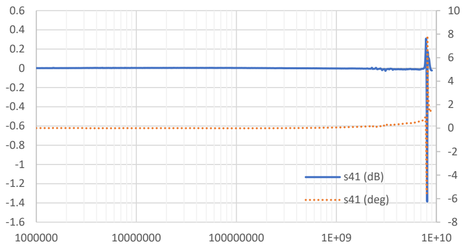
Bare 2x Through Coupon, Self de-embedded, IL
