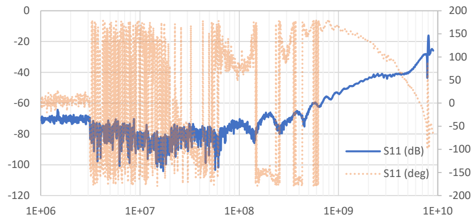
Bare 2x Through Coupon, Self de-embedded, RL
