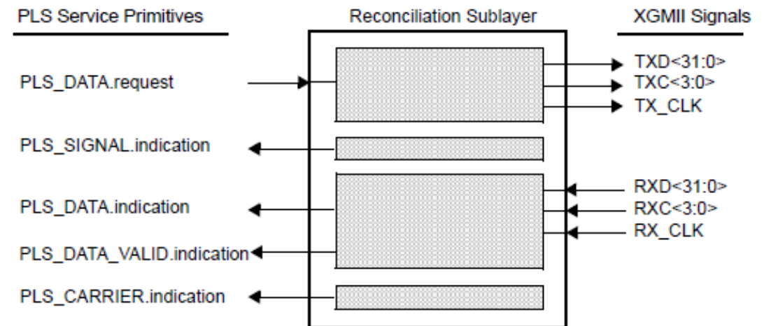
Figure 46–2—Reconciliation Sublayer (RS) inputs and outputs
