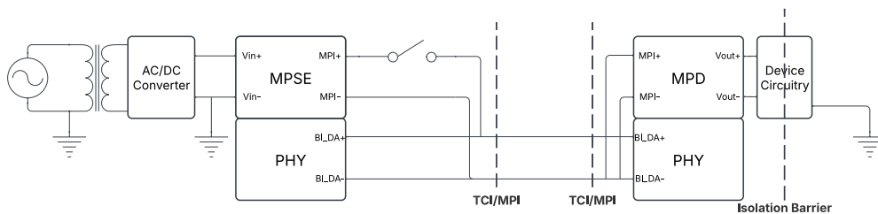
Figure J-2 Grounded MPoE System Diagram
