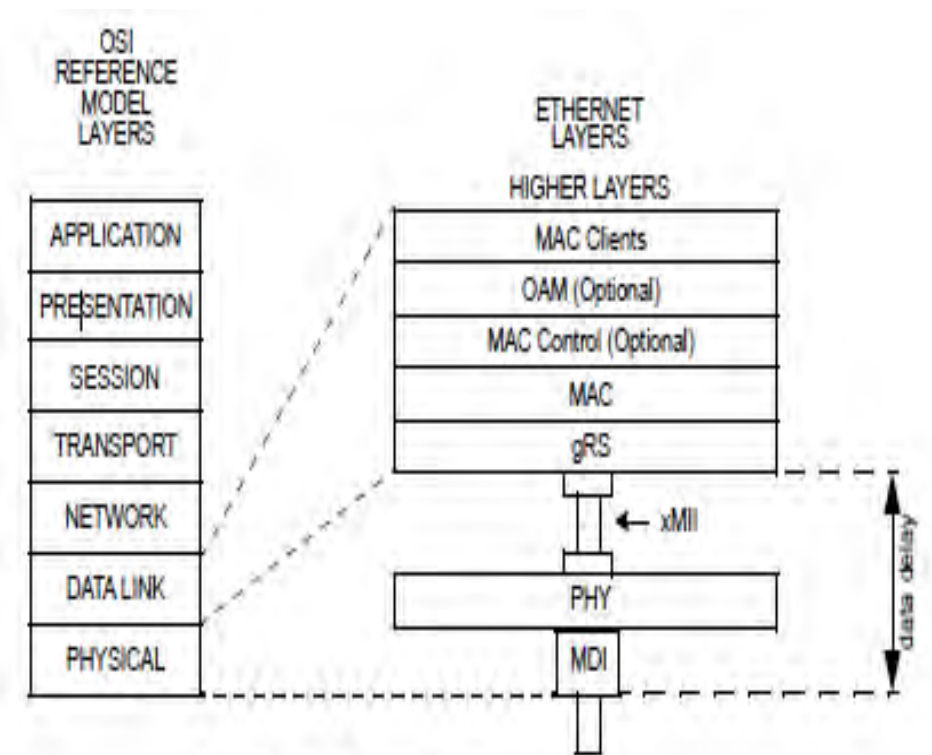
Figure 90-3—Data delay measurement
