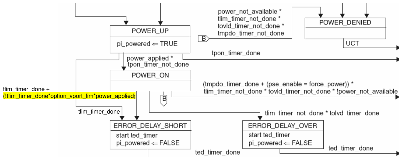
Figure 33–6—PSE state diagram
