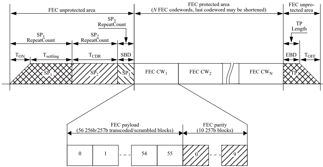
Figure 142-1—ONU burst structure, 3 zones
