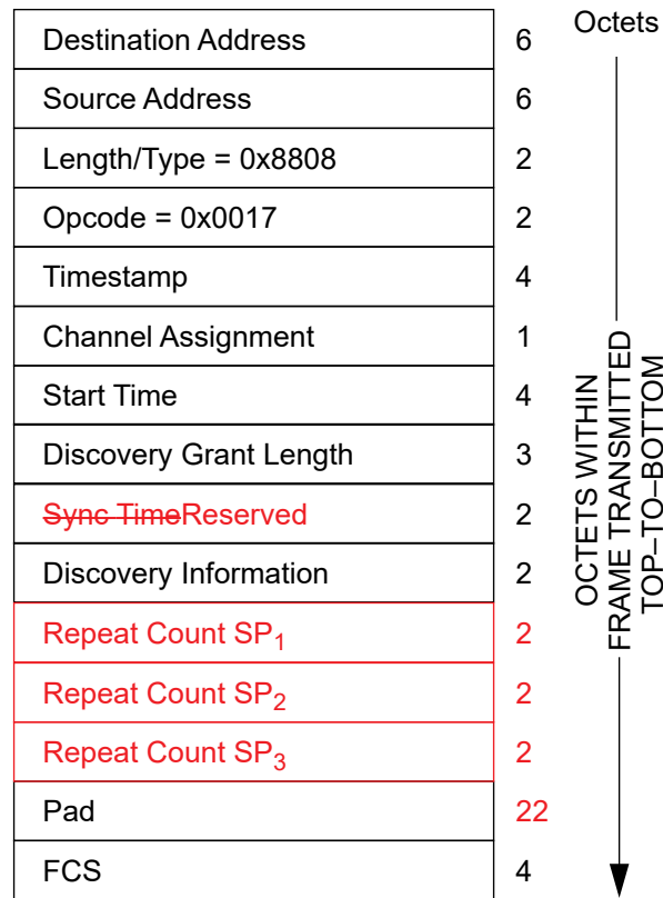
Figure 144-27—DISCOVERY_GATE MPCPDU
