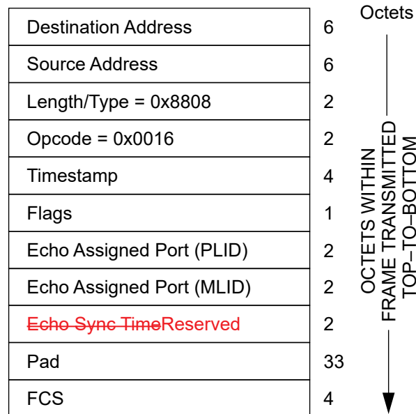
Figure 144–26—REGISTER_ACK MPCPDU
