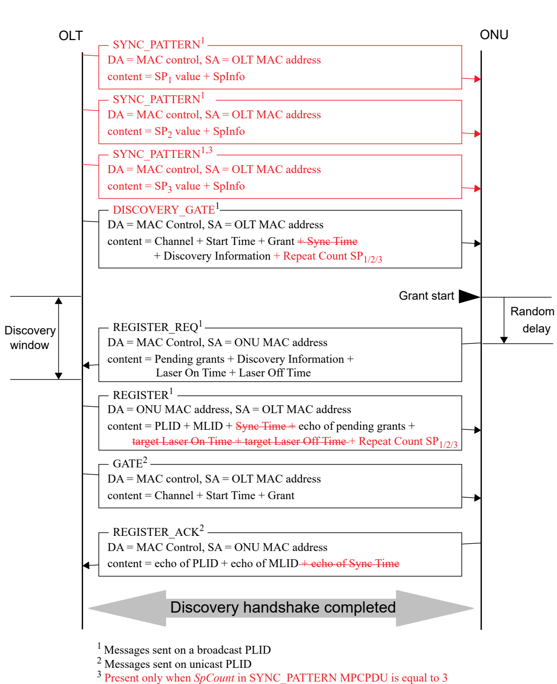
Figure 144-1—Discovery handshake message exchange
