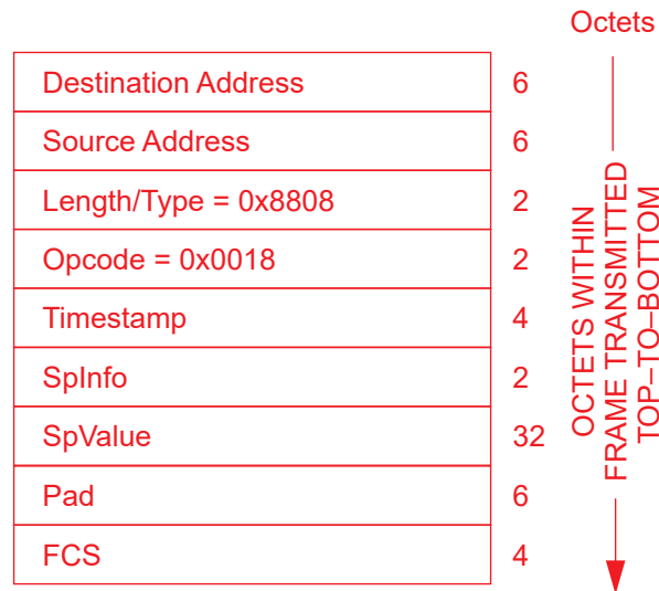
Figure 144-28—SYNC_PATTERN MPCPDU
