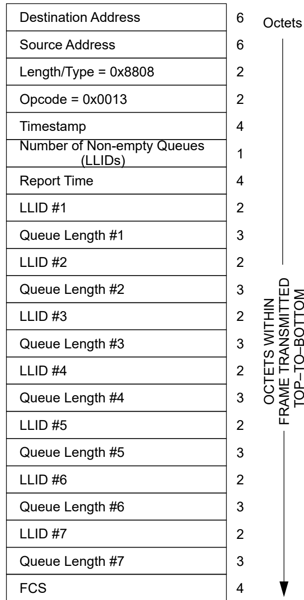
Figure 144-23—REPORT MPCPDU
