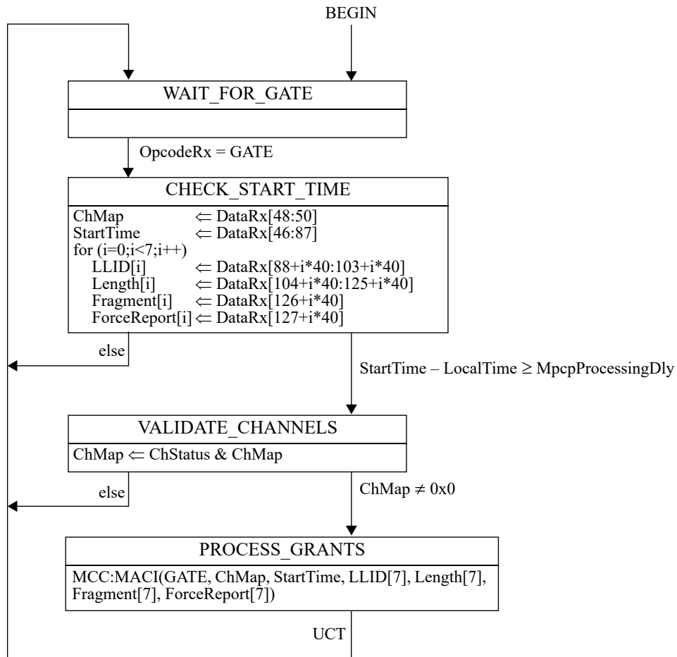
Figure 144–19—ONU GATE Reception Process state diagram
