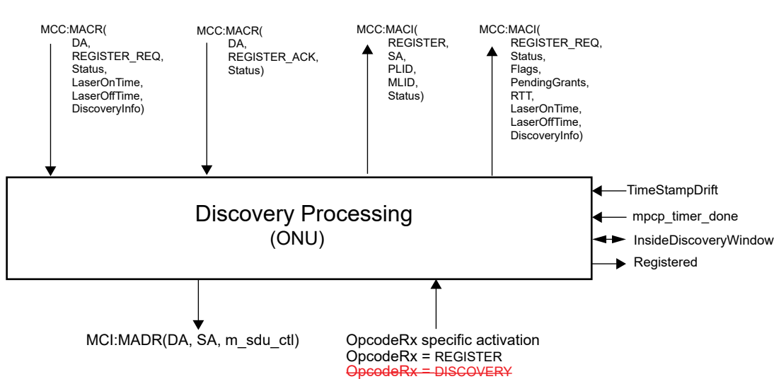
Figure 144-6—Discovery Processing service interfaces (ONU)
