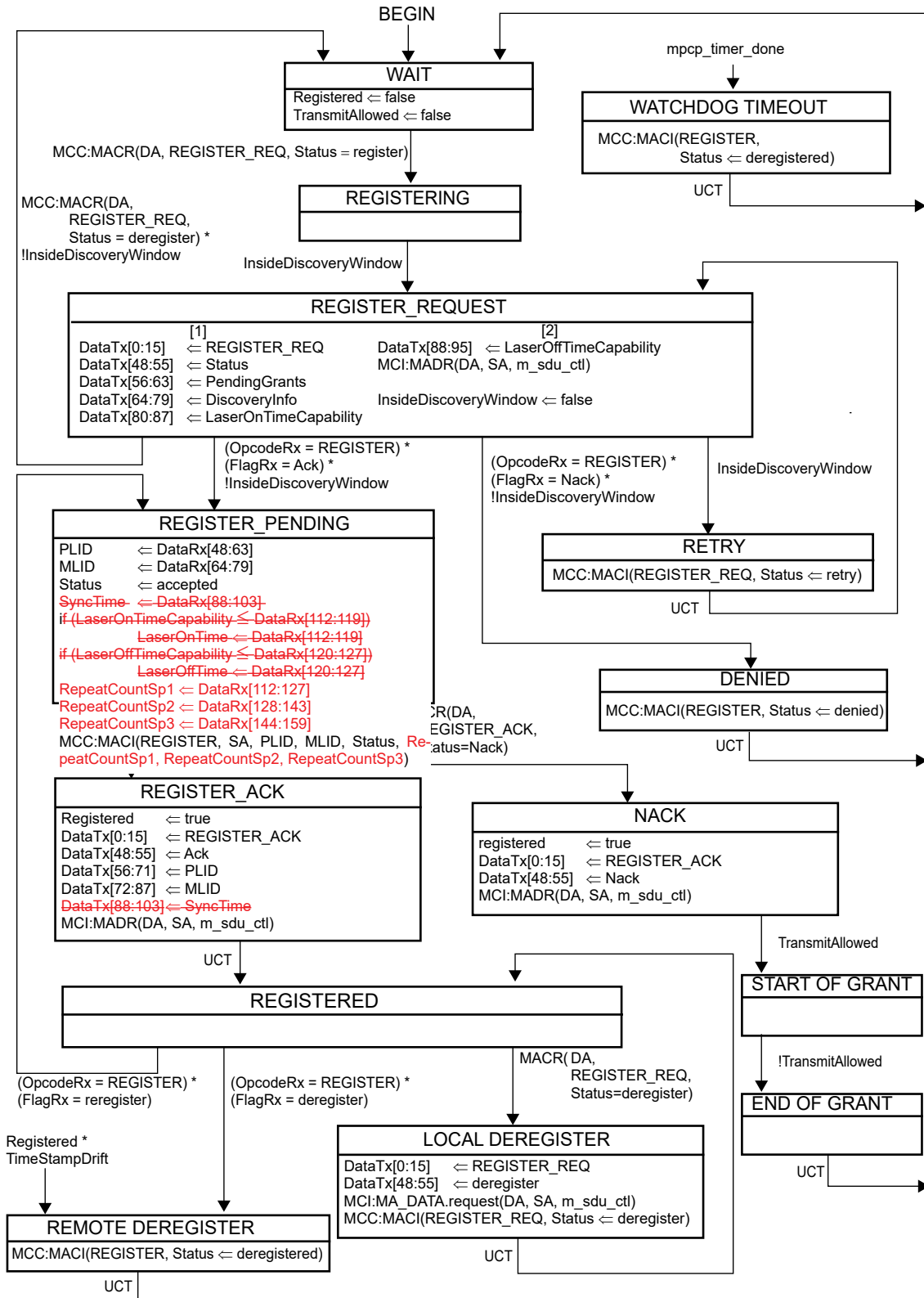
Figure 144-13—Discovery Processing ONU Registration state diagram
