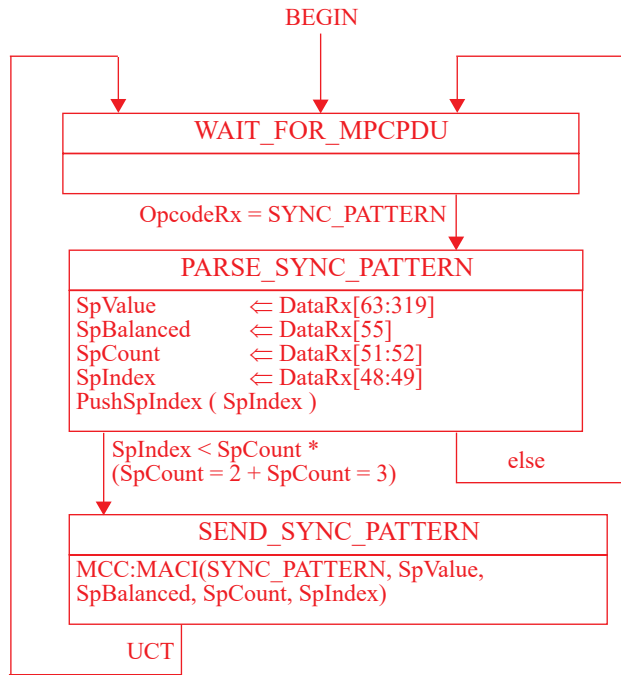
Figure 144–11—SYNC_PATTERN Validation ONU state diagram
