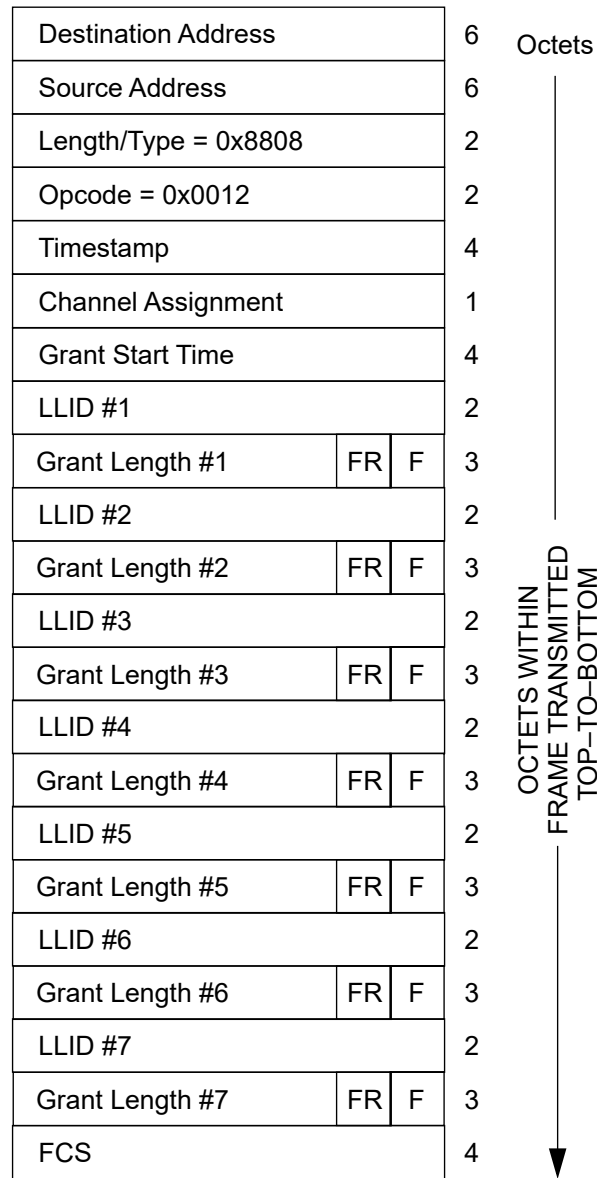
Figure 144-22—GATE MPCPDU
