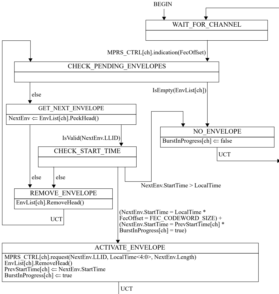
Figure 144–20—Envelope Activation Process state diagram
