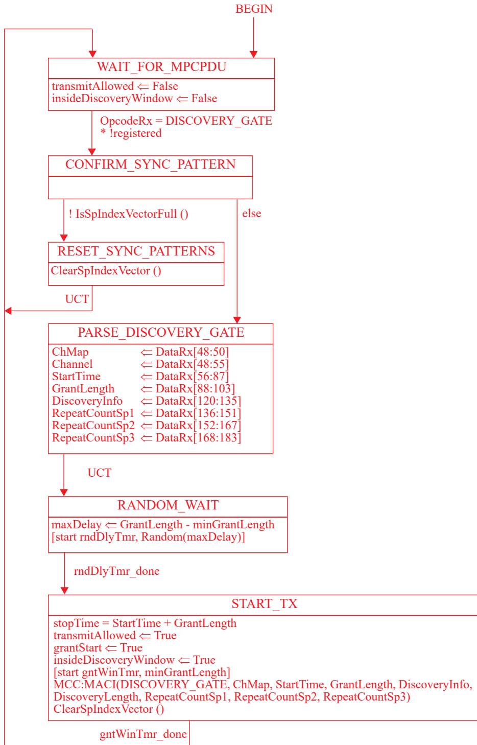
Figure 144–12—DISCOVERY_GATE Activation ONU state diagram
