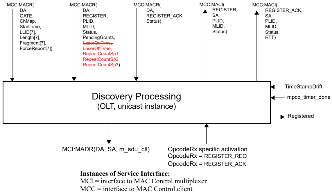
Figure 144-3—Discovery Processing service interfaces (OLT, unicast instance)
