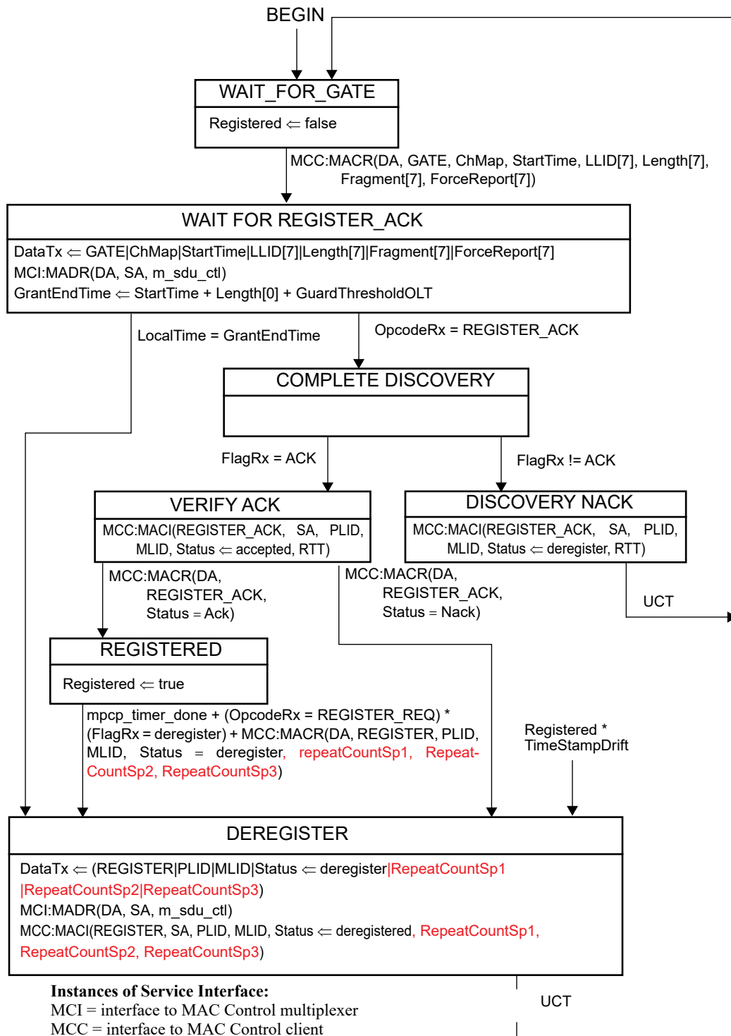
Figure 144–10—Discovery Processing OLT Final Registration state diagram
