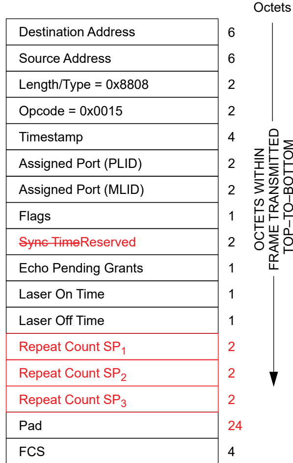
Figure 144-25—REGISTER MPCPDU
