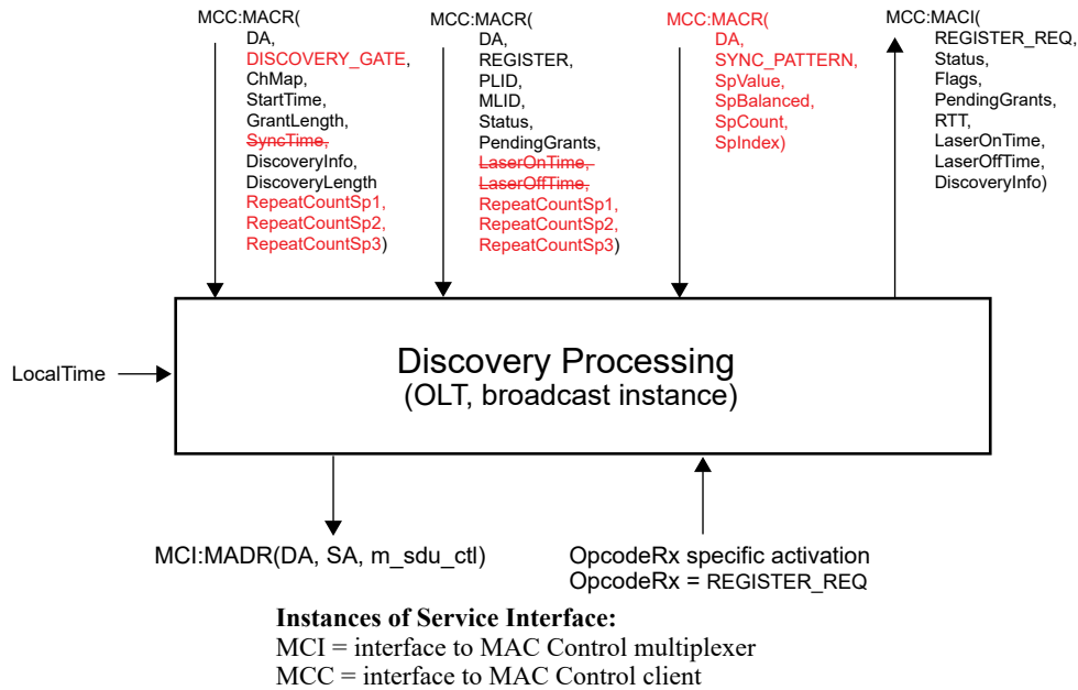
Figure 144-2—Discovery Processing service interfaces (OLT, broadcast instance)
