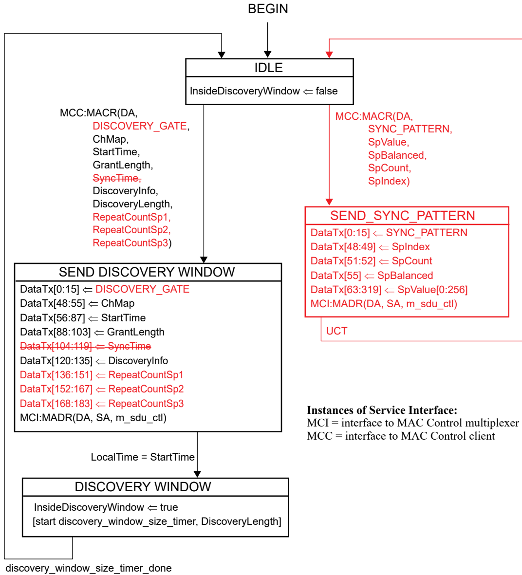
Figure 144-7—Discovery Processing OLT Window Setup state diagram
