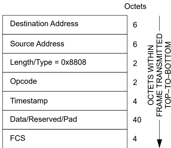
Figure 144–21—Generic MPCPDU
