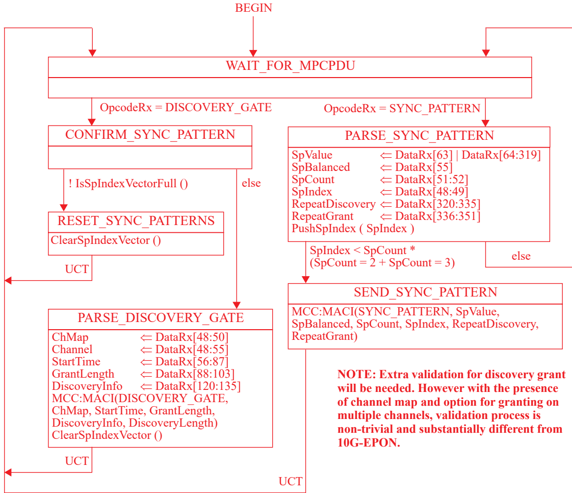
Figure 144–10—Discovery Initiation ONU state diagram
