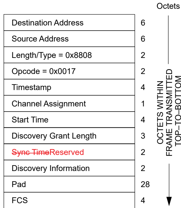
Figure 144-25—DISCOVERY_GATE MPCPDU
