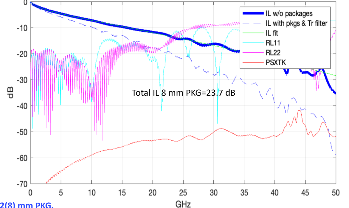
C2M_1218 --112G_cascaded_CDR6_Module_Thru_1_etch1100_TX3_Asic_Footprint Losses
