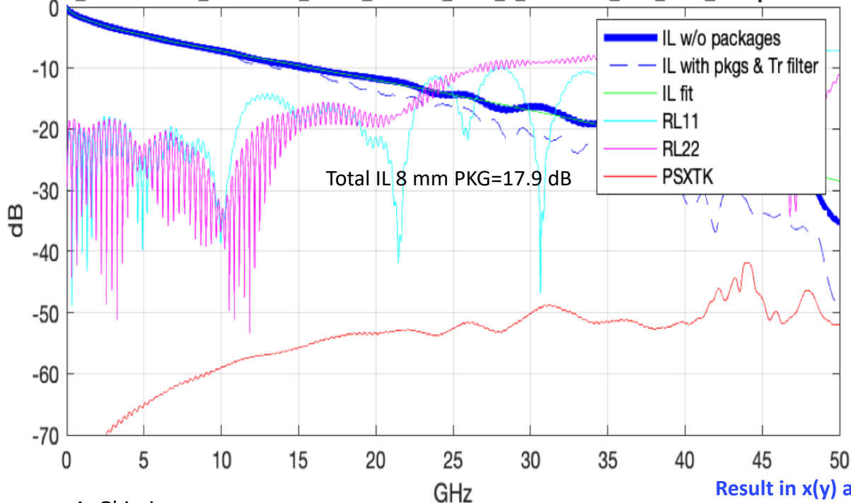
C2M_1218 --112G_cascaded_CDR6_Module_Thru_1_etch1100_TX3_Asic_Footprint Losses
