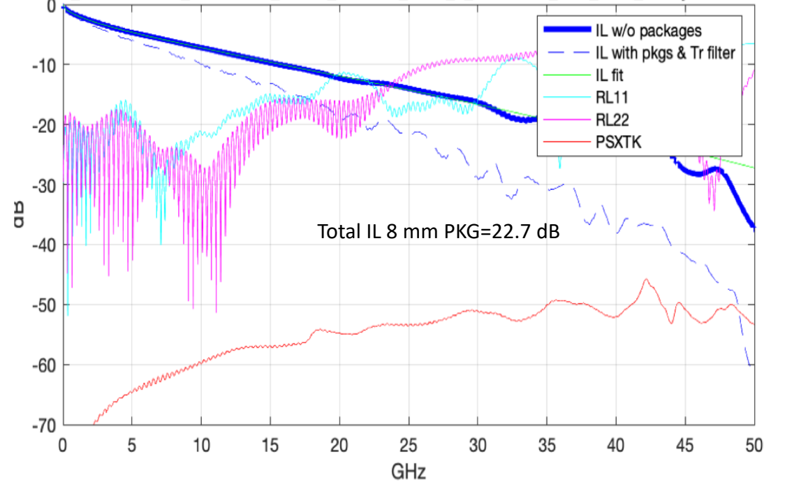
C2M_1218 --112G_cascaded_CDR6_Module_Thru_1_etch1100_TX7_Asic_Footprint Losses
