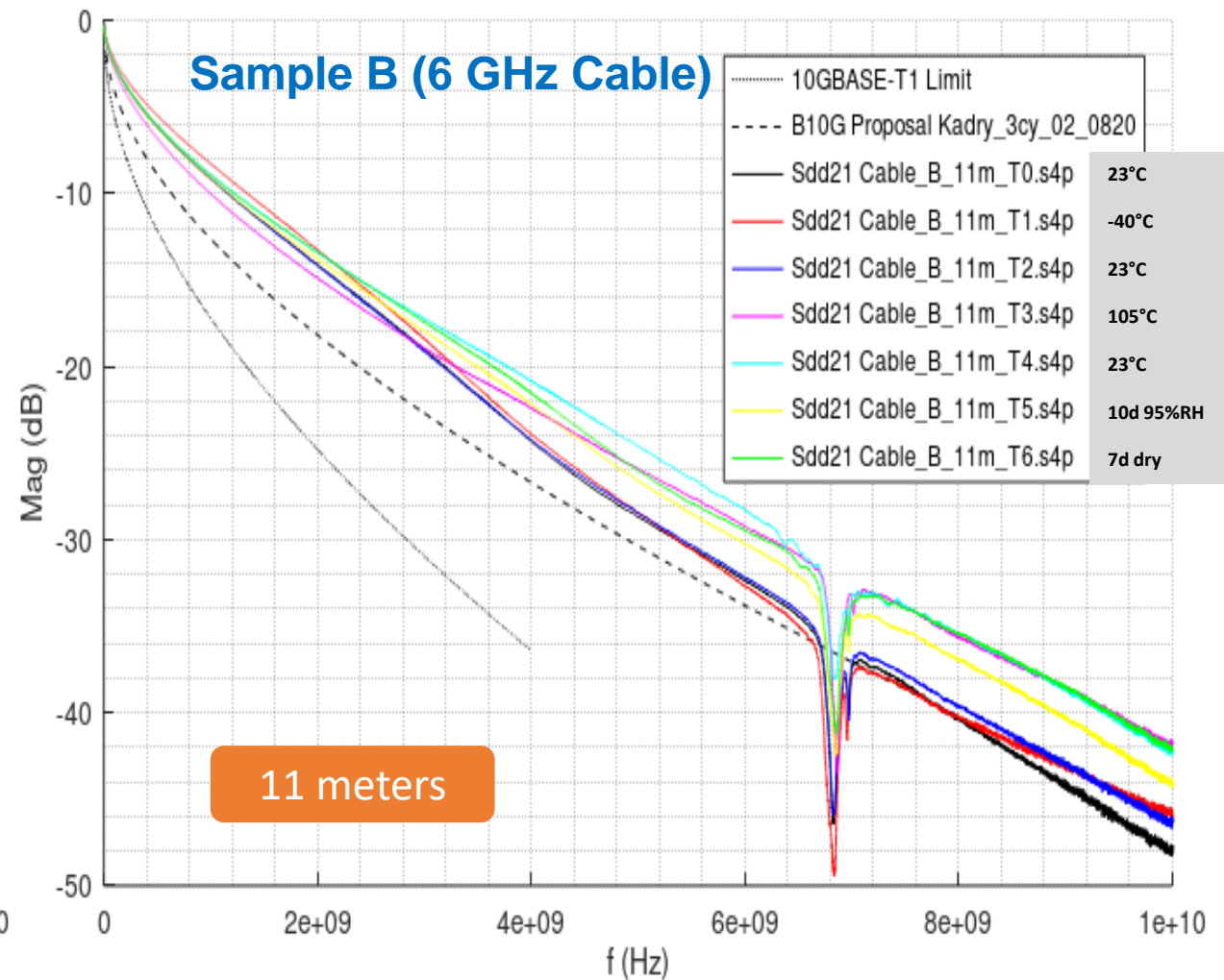
Insertion Loss (-dB)
