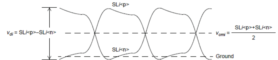
Figure 93-6—Transmitter output voltage definitions
