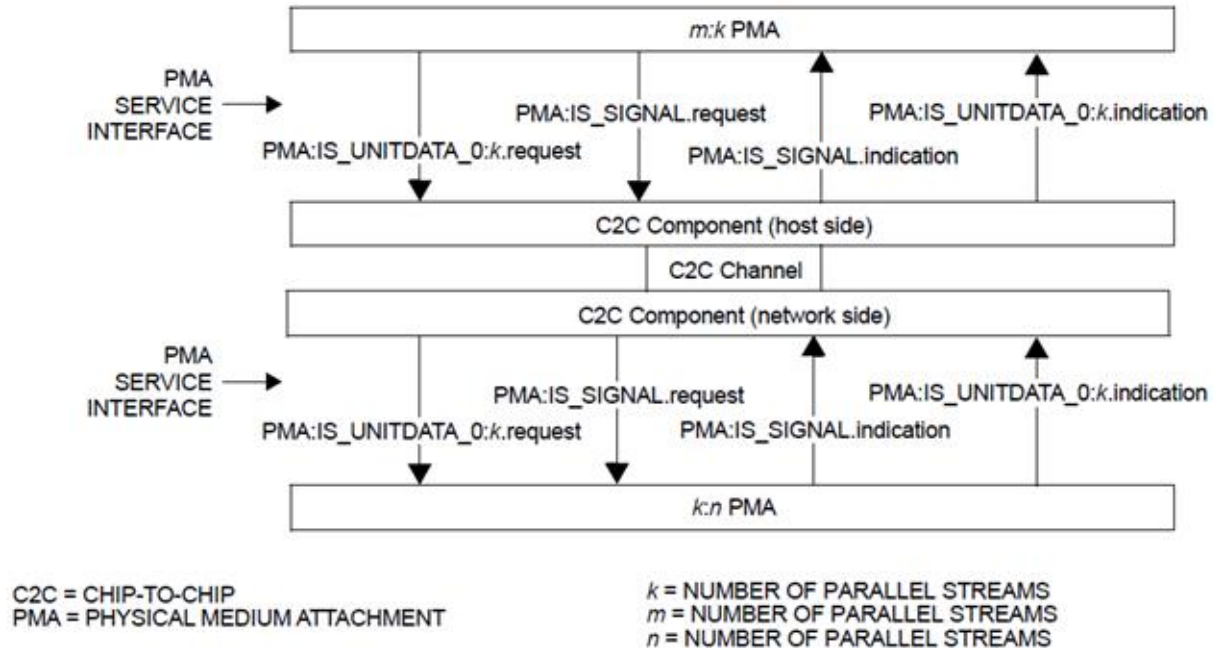
Figure 176C-3—Inter-sublayer service interfaces for a 200GAUI-1, 400GAUI-2, 800GAUI-4, or 1.6TAUI-8 C2C
