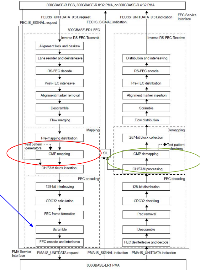
Figure 186-3—800GBASE-ER1 FEC functional block diagram
