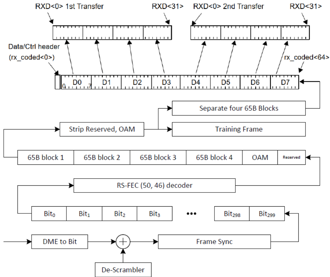
Figure 200-8—PCS Receive bit ordering for data mode and training mode
