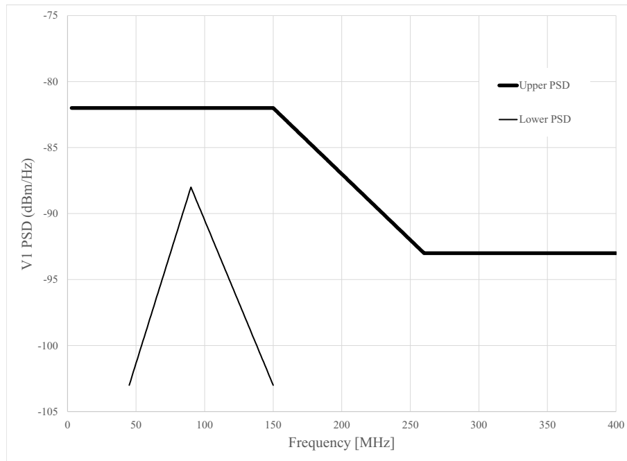
Figure 200-24—V1 100M Transmitter Power Spectral Density, upper and lower masks
