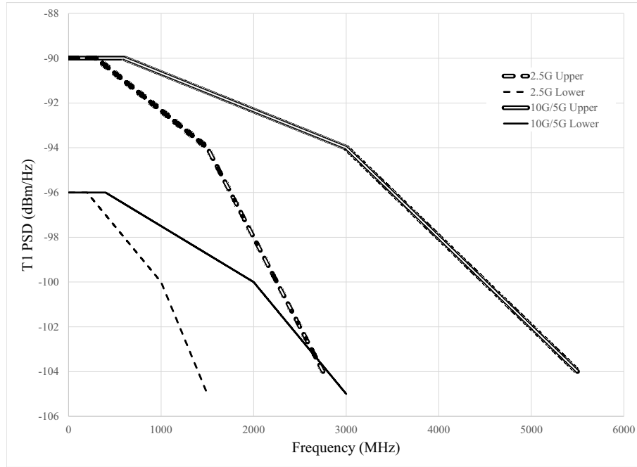
Figure 200-17—T1 MultiGTransmitter Power Spectral Density, upper and lower masks
