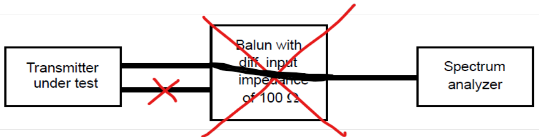
Figure 200-22—Transmitter test fixture 4 for power spectral density measurement and
