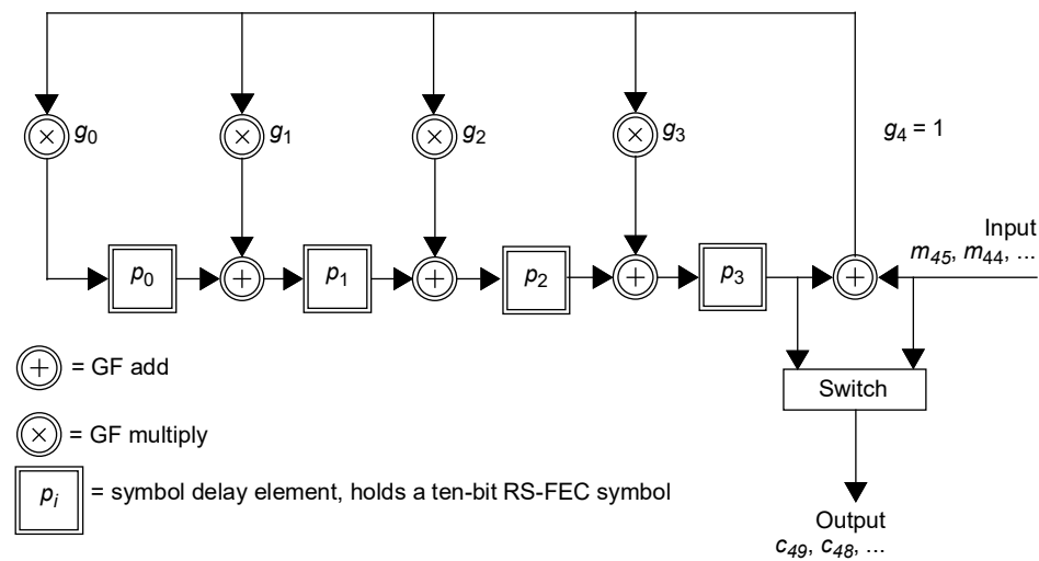
Figure 200–9—Reed-Solomon encoder functional model
