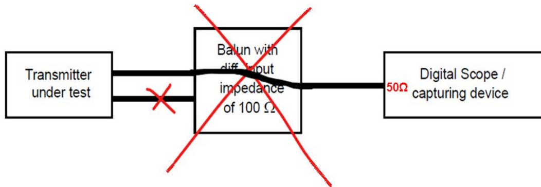
Figure 200-21—Transmitter test fixture 3 for MDI jitter measurement
