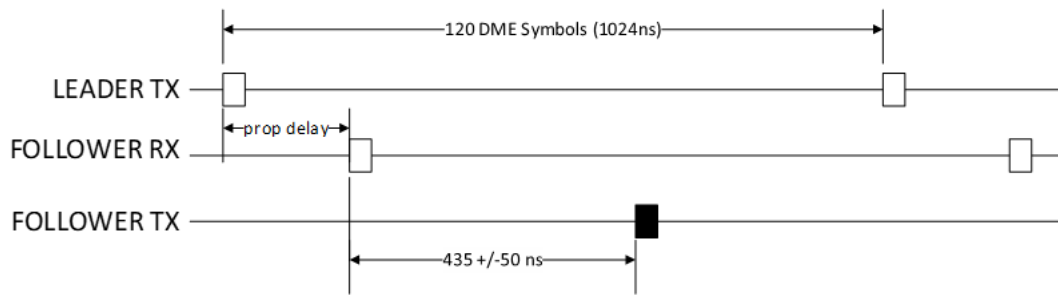
Figure 200–15—Link Synchronization timing
