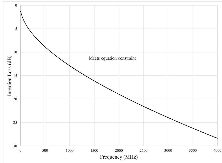
Figure 200–25—Insertion loss using Equation (200–9) for T1 and V1
