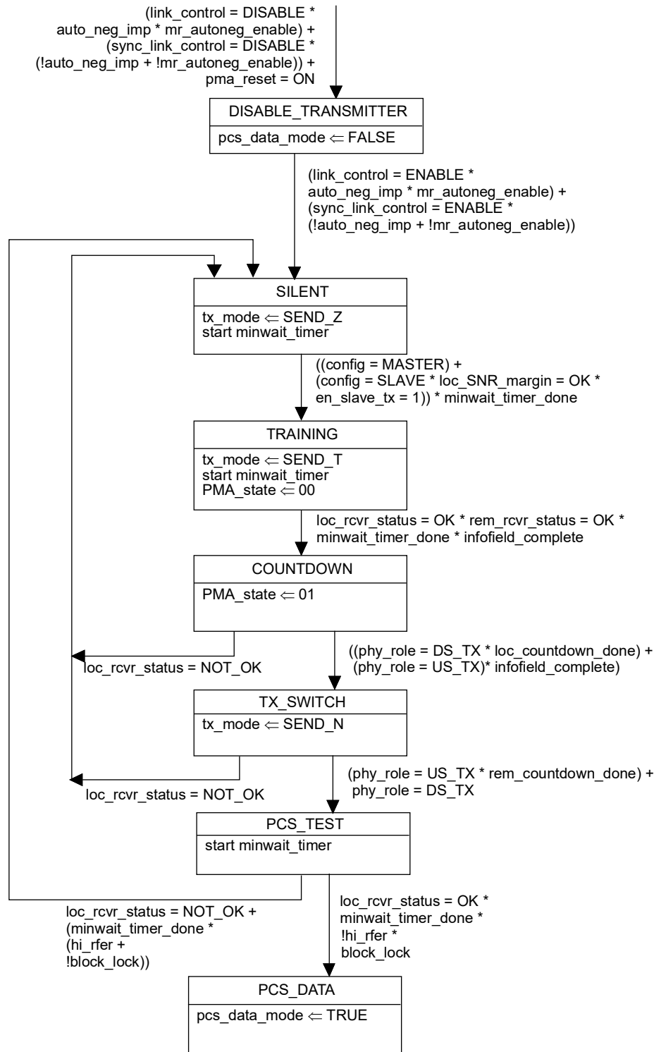
Figure 200–13—PHY Control state diagram
