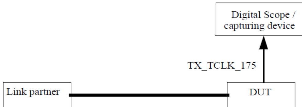
Figure 200–20—Transmitter test fixture 2 for MASTER and SLAVE clock jitter measurement
