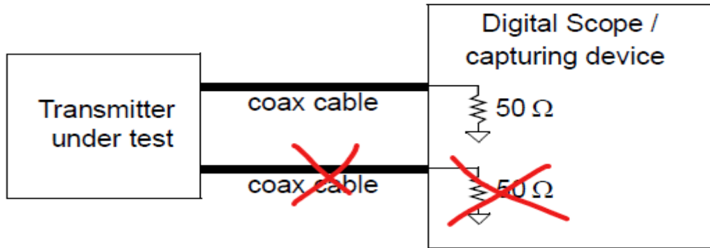
Figure 200–19—Transmitter test fixture 1 for transmitter droop measurement and
