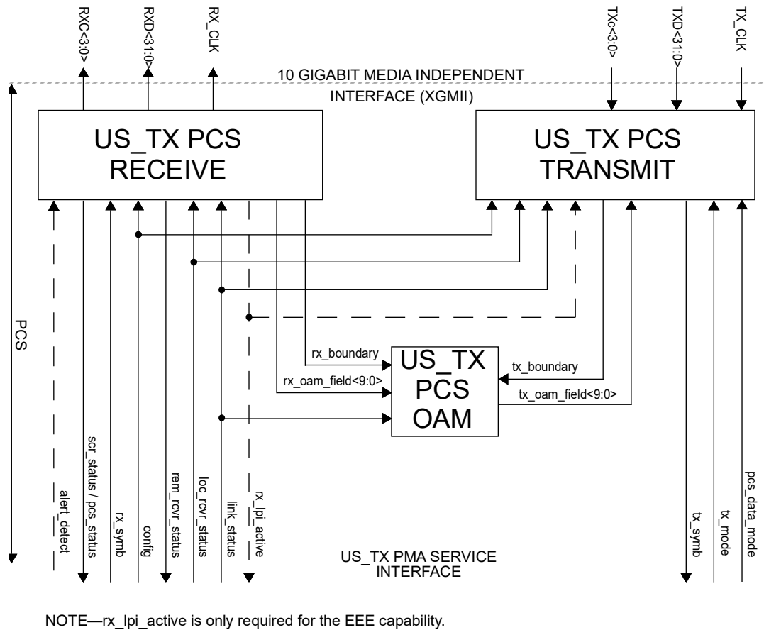
Figure 200-6—PCS reference diagram
