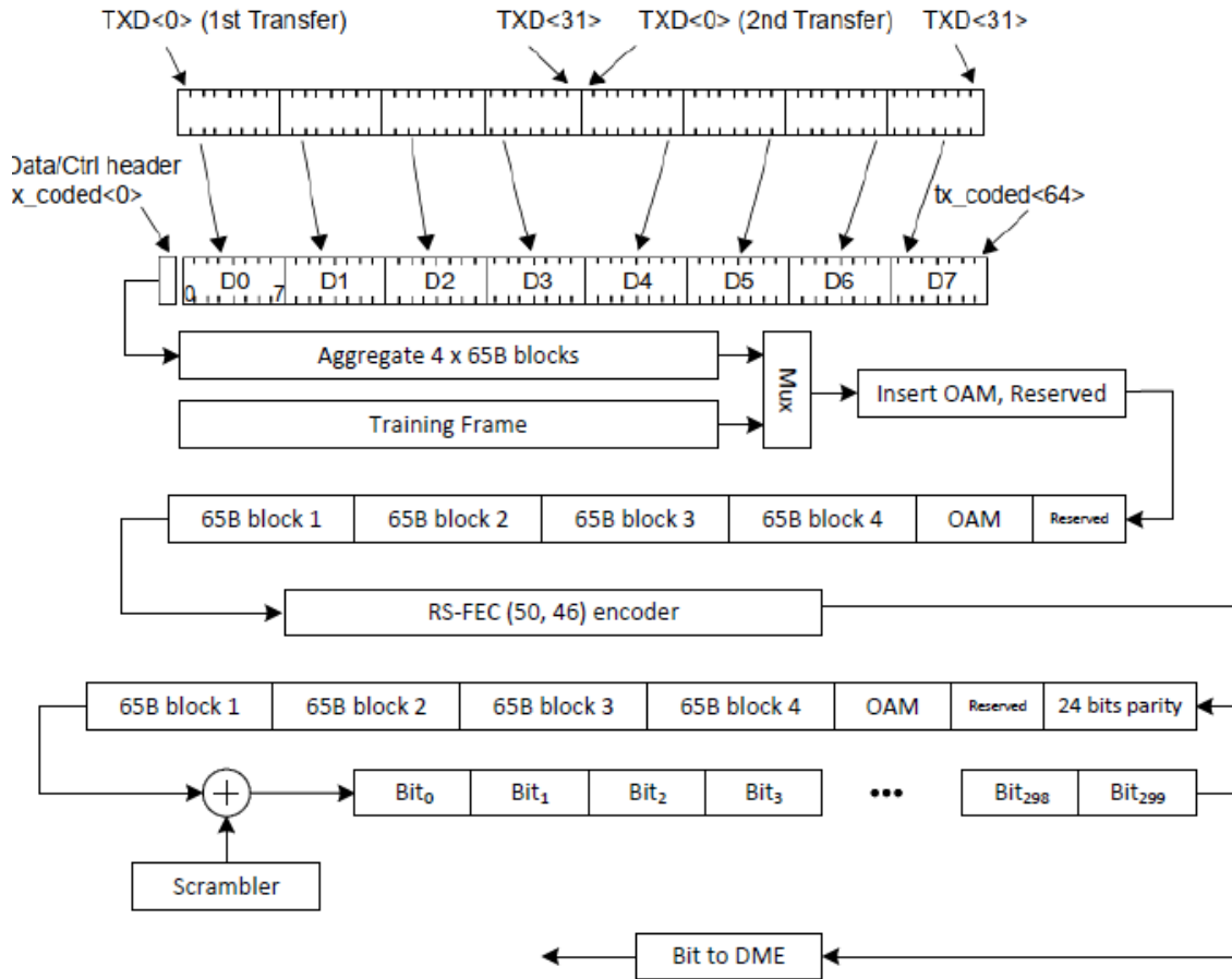
Figure 200-7—PCS Transmit bit ordering for data mode and training mode
