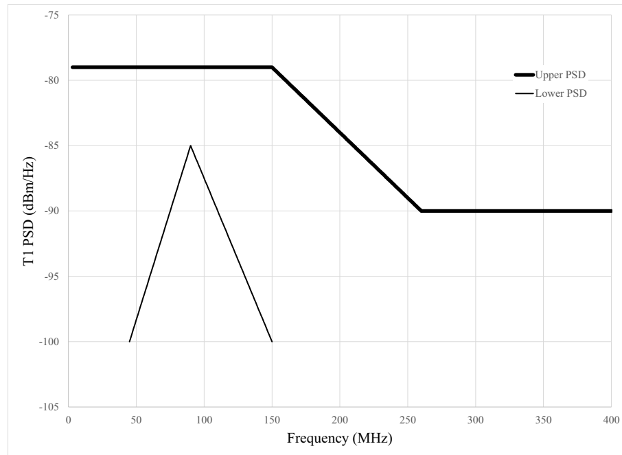
Figure 200-18—T1 100M Transmitter Power Spectral Density, upper and lower masks
