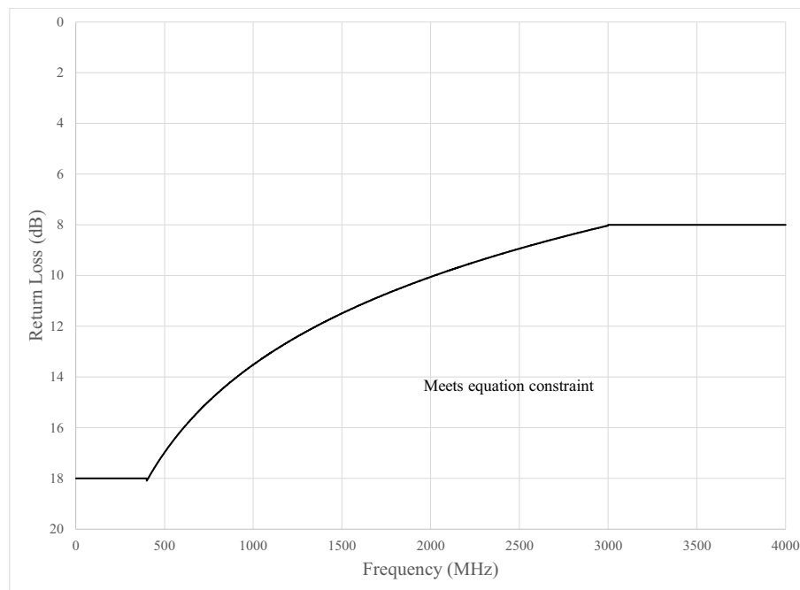
Figure 200–26—Return loss using Equation (200–11) for T1 and V1
