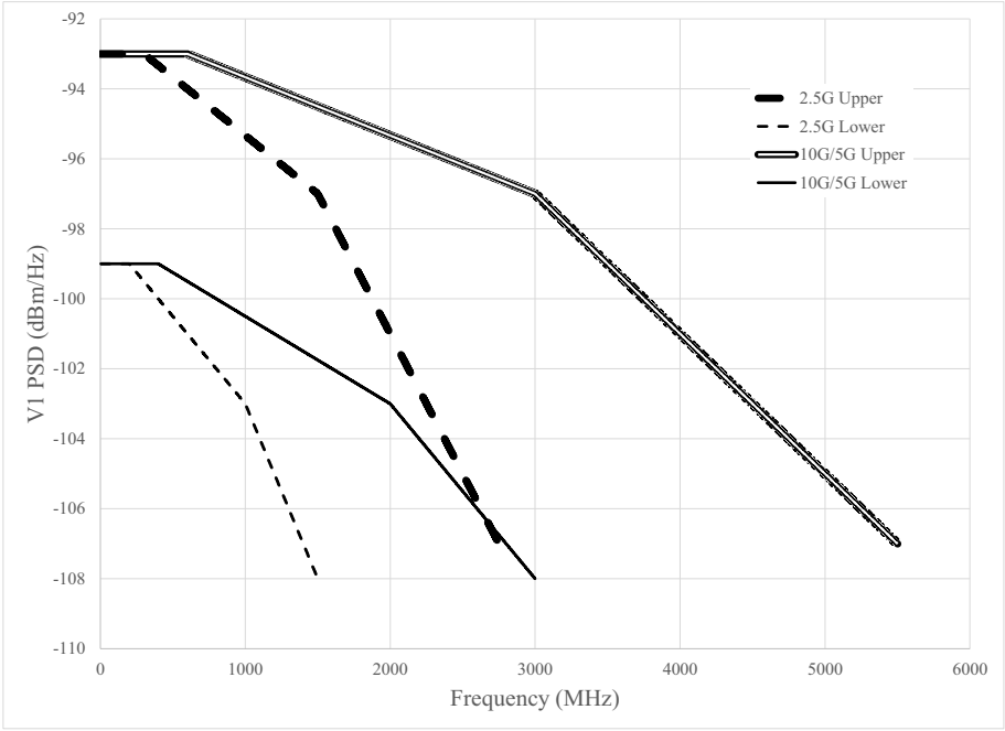
Figure 200-23—V1 MultiGTransmitter Power Spectral Density, upper and lower masks
