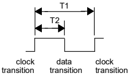
Figure 200–10—DME encoding scheme
