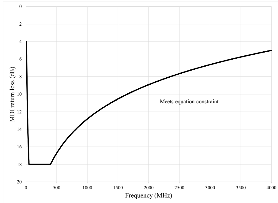
Figure 200–27—MDI return loss using Equation (200–12)
