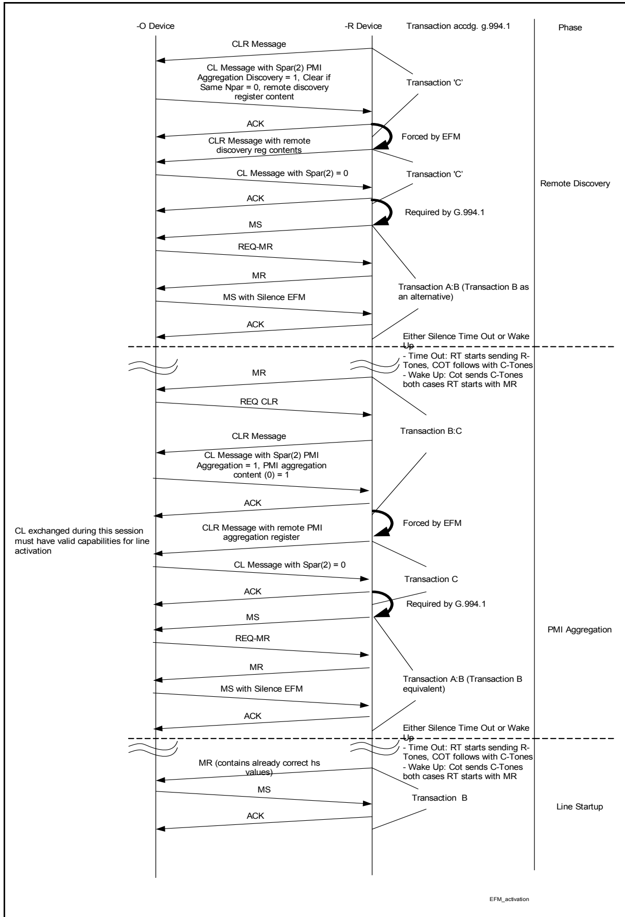
Figure 1: EFM activation sequence
