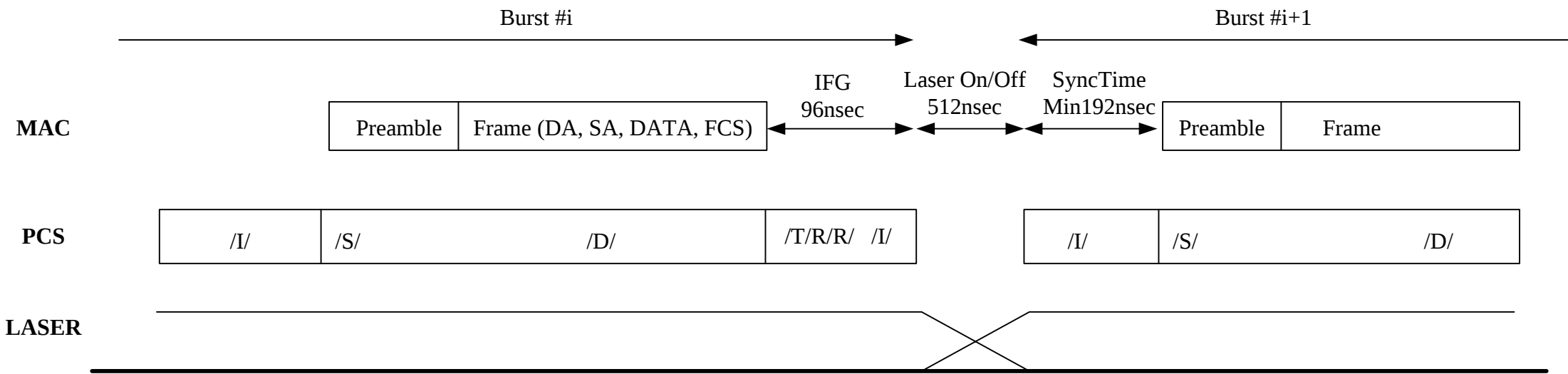
Fig 2: Between bursts. IFG is the end sequence of a burst
