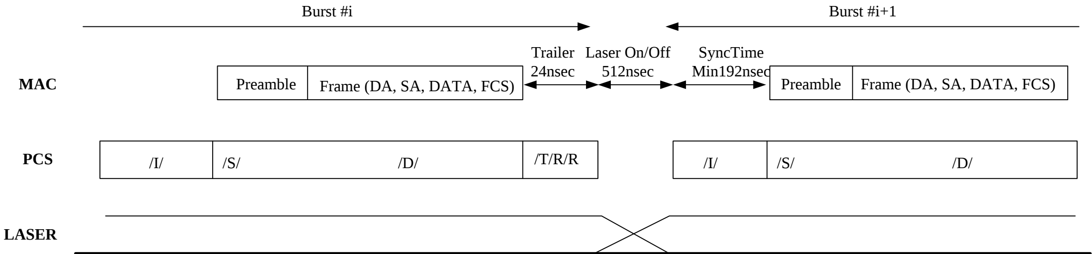
Fig 1: Between bursts. PCS trailer is the end sequence of a burst.
